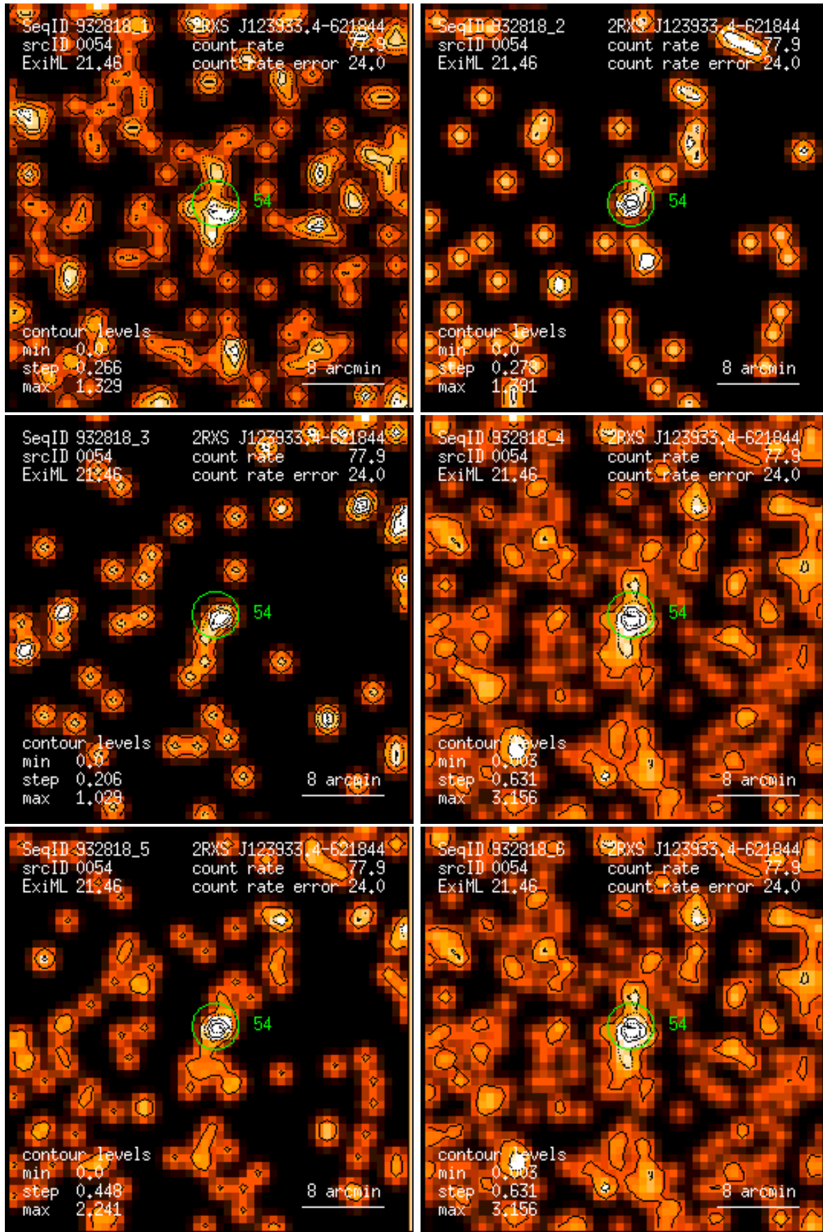
Figure 54: RASS 932818: detection 0054: band rate images, Gaussian filter: (1) PSPC channels 11 – 41, (2) 52 – 90, (3) 91 – 201, (4) 11 – 235, (5) 52 – 201, (6) 11 – 201. Broad band rates in counts/ks. Band rate contour levels in counts/ks/arcmin 2 .
