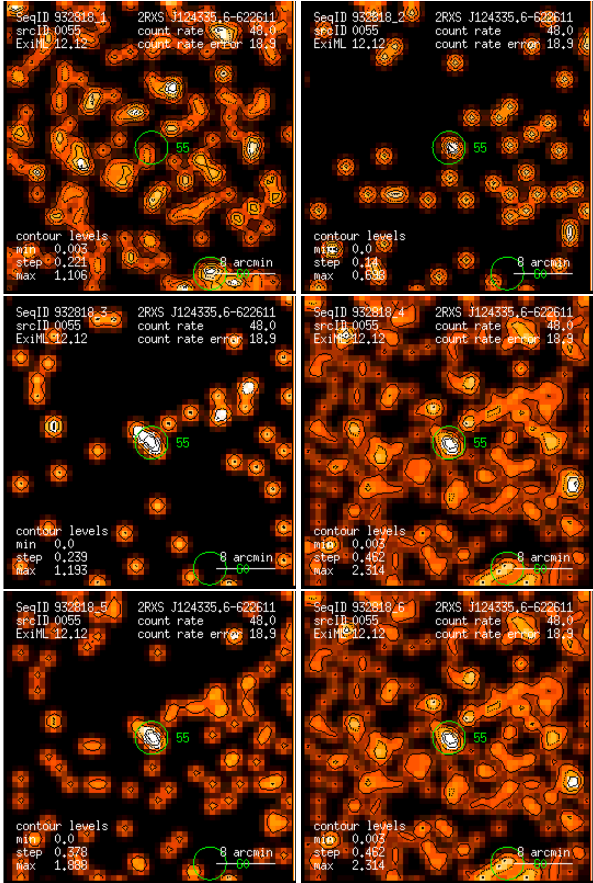
Figure 55: RASS 932818: detection 0055: band rate images, Gaussian filter: (1) PSPC channels 11 – 41, (2) 52 – 90, (3) 91 – 201, (4) 11 – 235, (5) 52 – 201, (6) 11 – 201. Broad band rates in counts/ks. Band rate contour levels in counts/ks/arcmin 2 .
