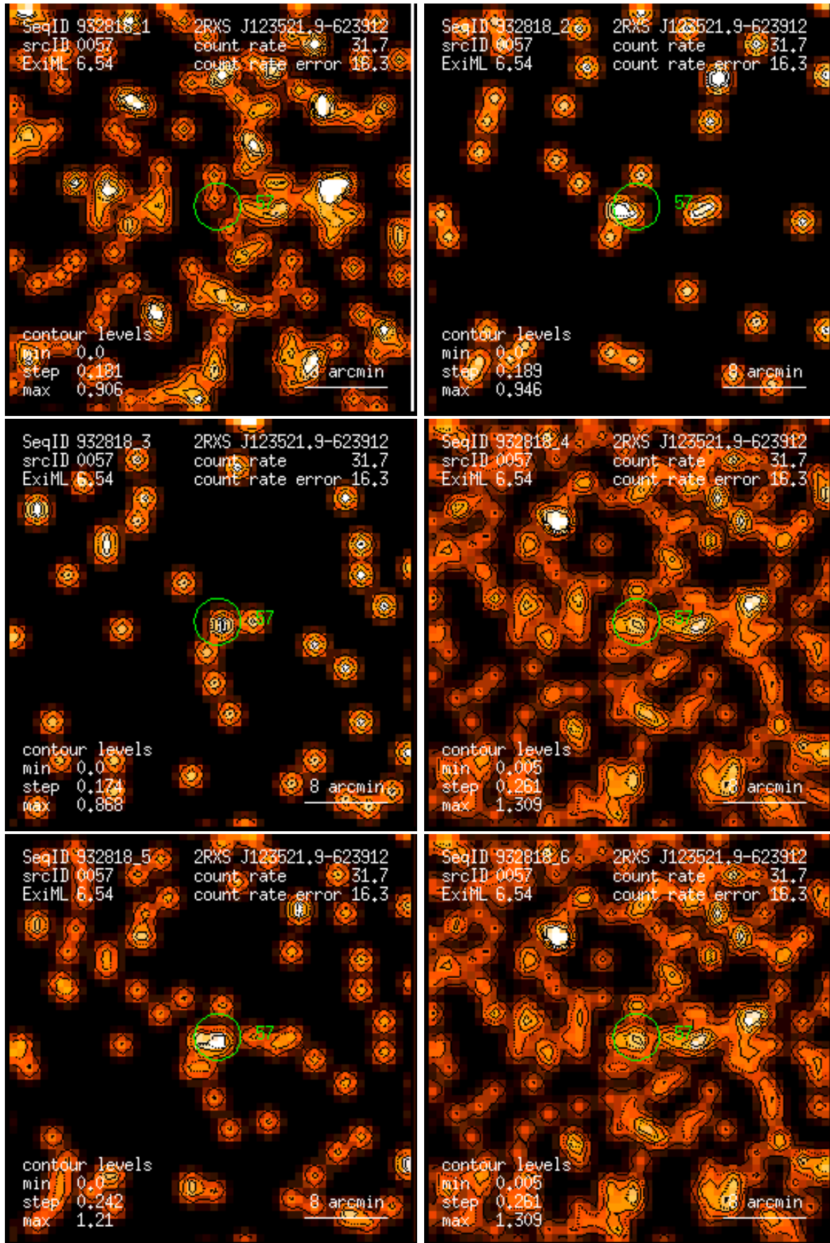
Figure 57: RASS 932818: detection 0057: band rate images, Gaussian filter: (1) PSPC channels 11 – 41, (2) 52 – 90, (3) 91 – 201, (4) 11 – 235, (5) 52 – 201, (6) 11 – 201. Broad band rates in counts/ks. Band rate contour levels in counts/ks/arcmin 2 .
