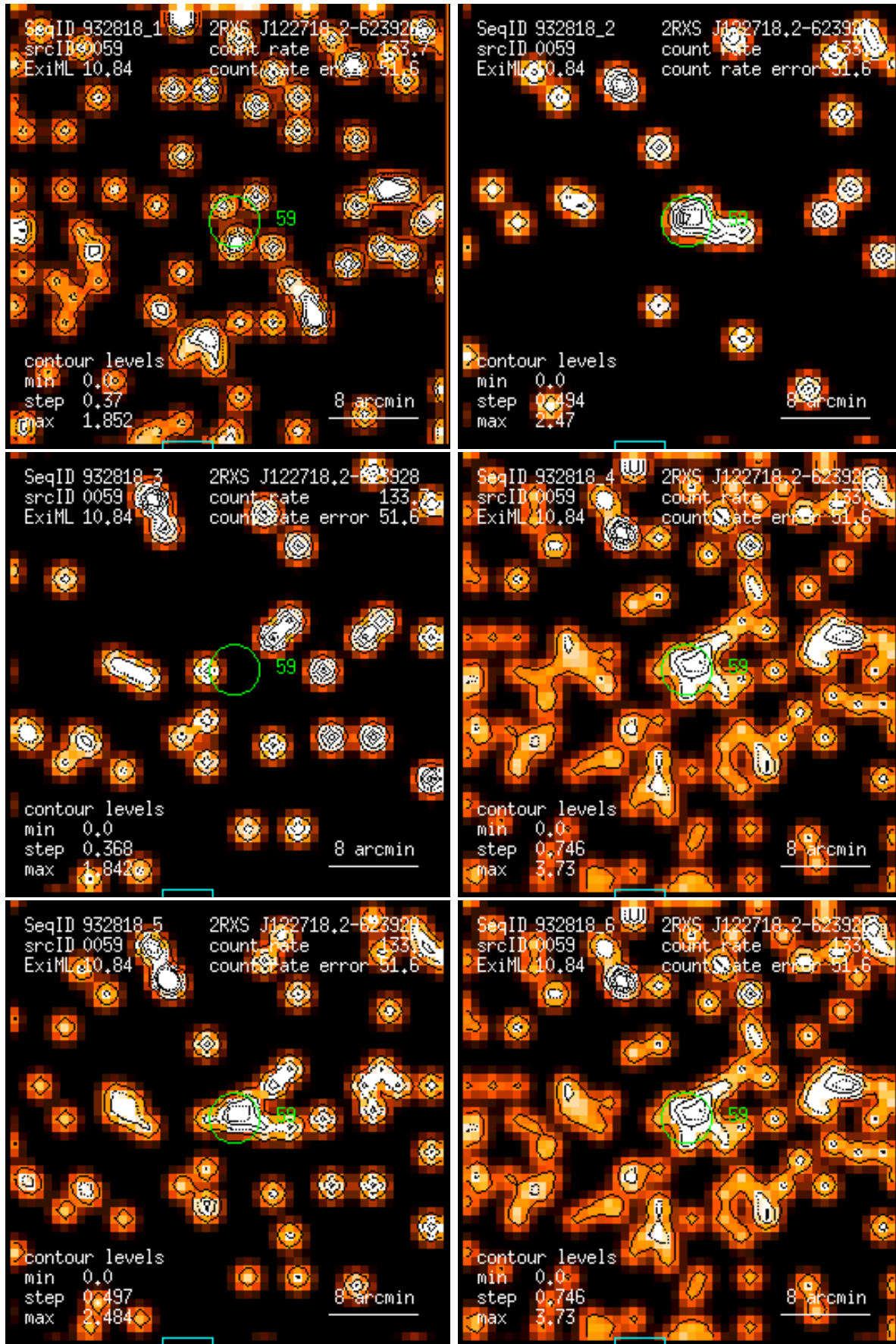
Figure 59: RASS 932818: detection 0059: band rate images, Gaussian filter: (1) PSPC channels 11 – 41, (2) 52 – 90, (3) 91 – 201, (4) 11 – 235, (5) 52 – 201, (6) 11 – 201. Broad band rates in counts/ks. Band rate contour levels in counts/ks/arcmin 2 .
