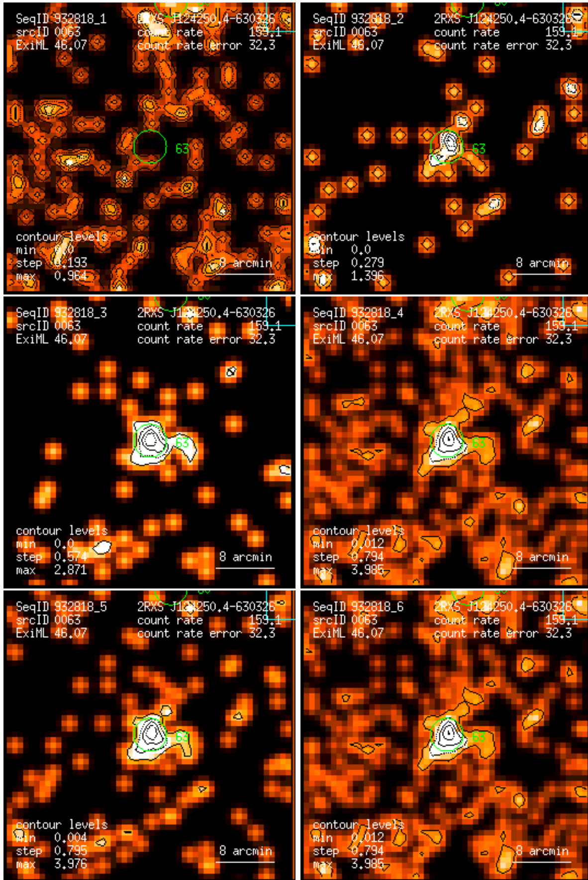
Figure 63: RASS 932818: detection 0063: band rate images, Gaussian filter: (1) PSPC channels 11 – 41, (2) 52 – 90, (3) 91 – 201, (4) 11 – 235, (5) 52 – 201, (6) 11 – 201. Broad band rates in counts/ks. Band rate contour levels in counts/ks/arcmin 2 .
