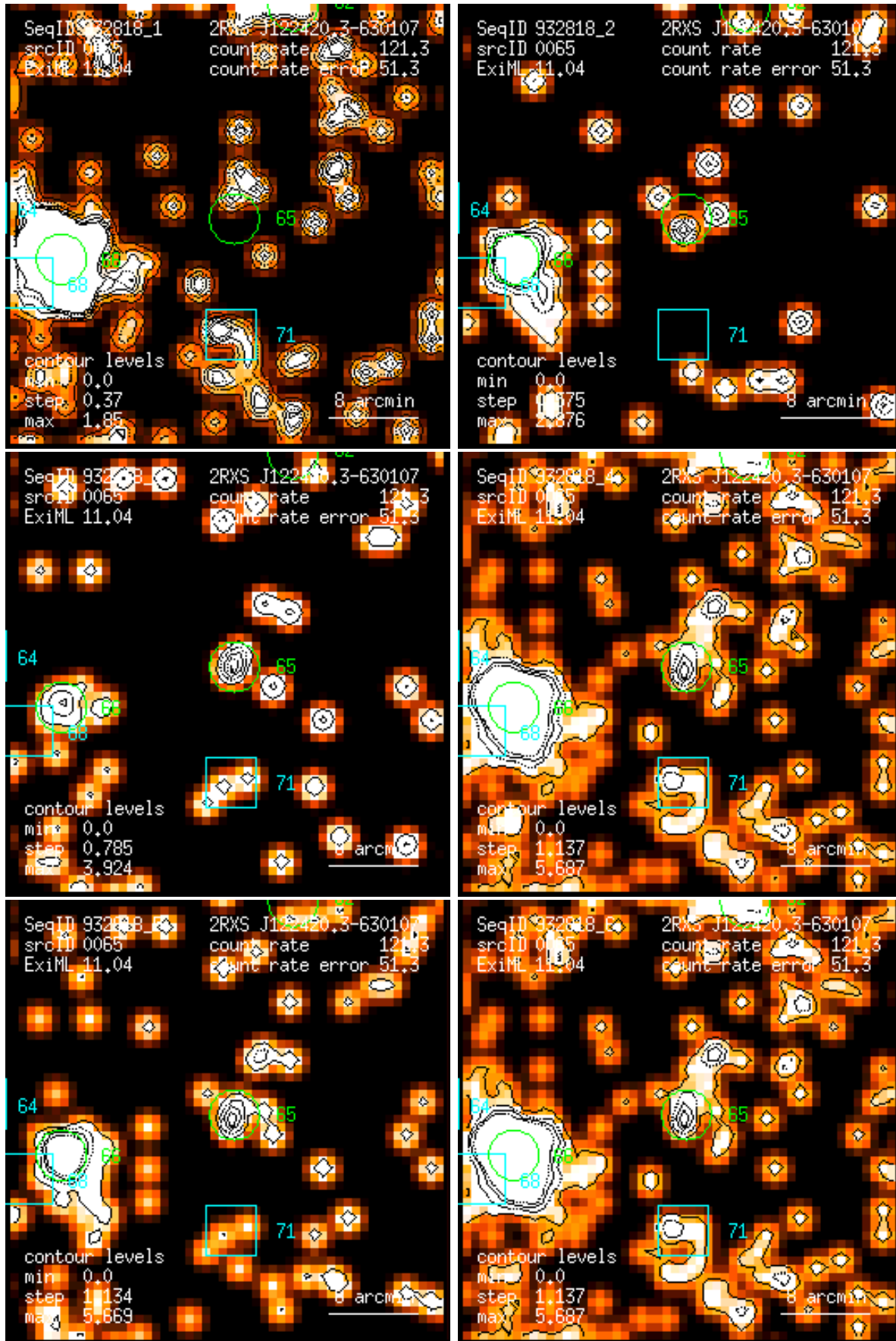
Figure 65: RASS 932818: detection 0065: band rate images, Gaussian filter: (1) PSPC channels 11 – 41, (2) 52 – 90, (3) 91 – 201, (4) 11 – 235, (5) 52 – 201, (6) 11 – 201. Broad band rates in counts/ks. Band rate contour levels in counts/ks/arcmin 2 .
