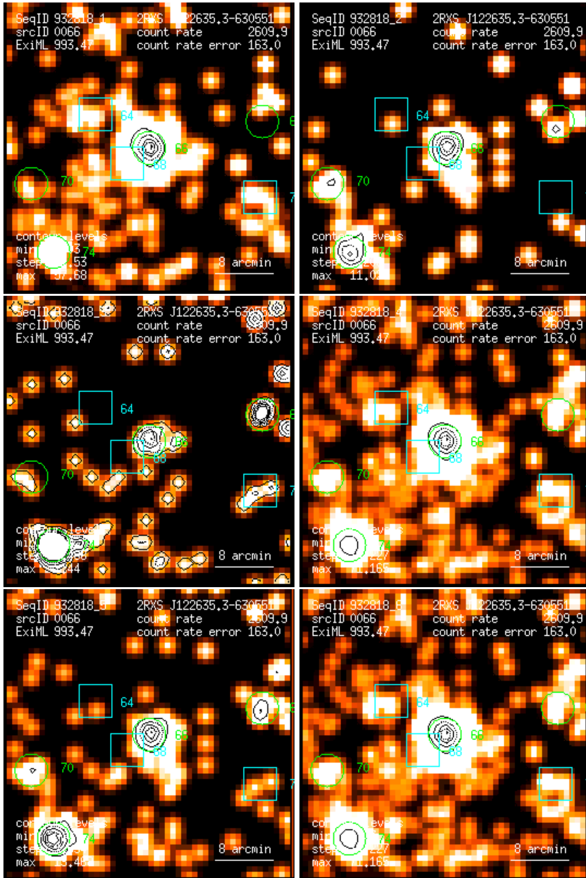
Figure 66: RASS 932818: detection 0066: band rate images, Gaussian filter: (1) PSPC channels 11 – 41, (2) 52 – 90, (3) 91 – 201, (4) 11 – 235, (5) 52 – 201, (6) 11 – 201. Broad band rates in counts/ks. Band rate contour levels in counts/ks/arcmin 2 .
