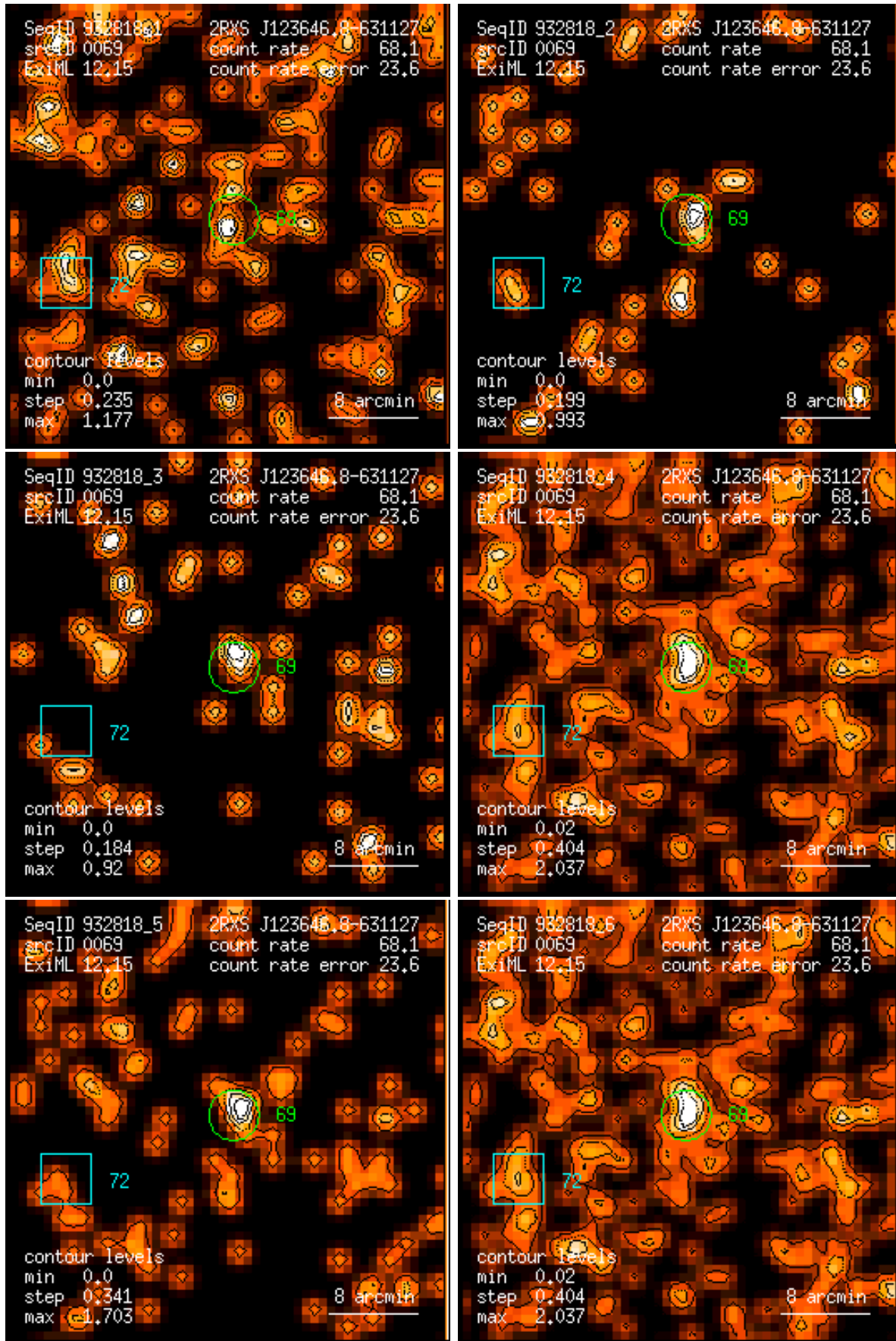
Figure 69: RASS 932818: detection 0069: band rate images, Gaussian filter: (1) PSPC channels 11 – 41, (2) 52 – 90, (3) 91 – 201, (4) 11 – 235, (5) 52 – 201, (6) 11 – 201. Broad band rates in counts/ks. Band rate contour levels in counts/ks/arcmin 2 .
