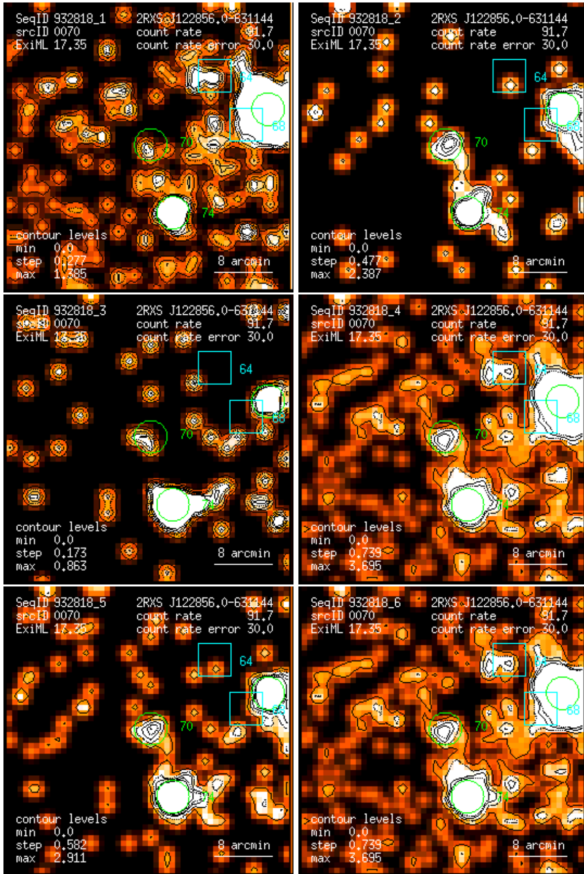
Figure 70: RASS 932818: detection 0070: band rate images, Gaussian filter: (1) PSPC channels 11 – 41, (2) 52 – 90, (3) 91 – 201, (4) 11 – 235, (5) 52 – 201, (6) 11 – 201. Broad band rates in counts/ks. Band rate contour levels in counts/ks/arcmin 2 .
