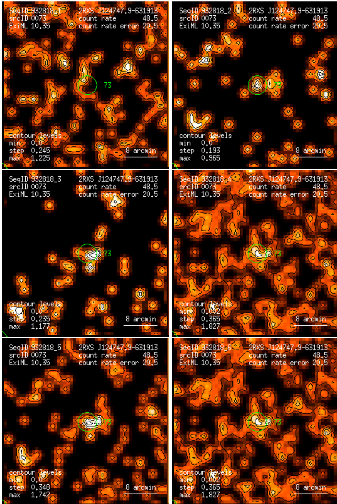
Figure 73: RASS 932818: detection 0073: band rate images, Gaussian filter: (1) PSPC channels 11 – 41, (2) 52 – 90, (3) 91 – 201, (4) 11 – 235, (5) 52 – 201, (6) 11 – 201. Broad band rates in counts/ks. Band rate contour levels in counts/ks/arcmin 2 .
