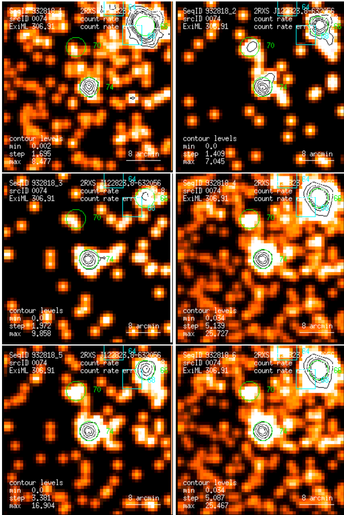
Figure 74: RASS 932818: detection 0074: band rate images, Gaussian filter: (1) PSPC channels 11 – 41, (2) 52 – 90, (3) 91 – 201, (4) 11 – 235, (5) 52 – 201, (6) 11 – 201. Broad band rates in counts/ks. Band rate contour levels in counts/ks/arcmin 2 .
