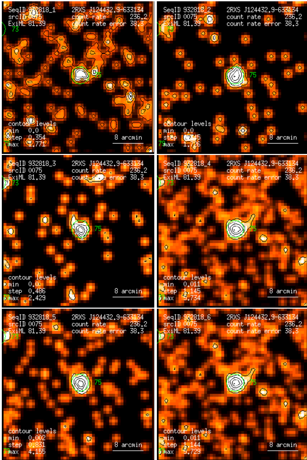
Figure 75: RASS 932818: detection 0075: band rate images, Gaussian filter: (1) PSPC channels 11 – 41, (2) 52 – 90, (3) 91 – 201, (4) 11 – 235, (5) 52 – 201, (6) 11 – 201. Broad band rates in counts/ks. Band rate contour levels in counts/ks/arcmin 2 .
