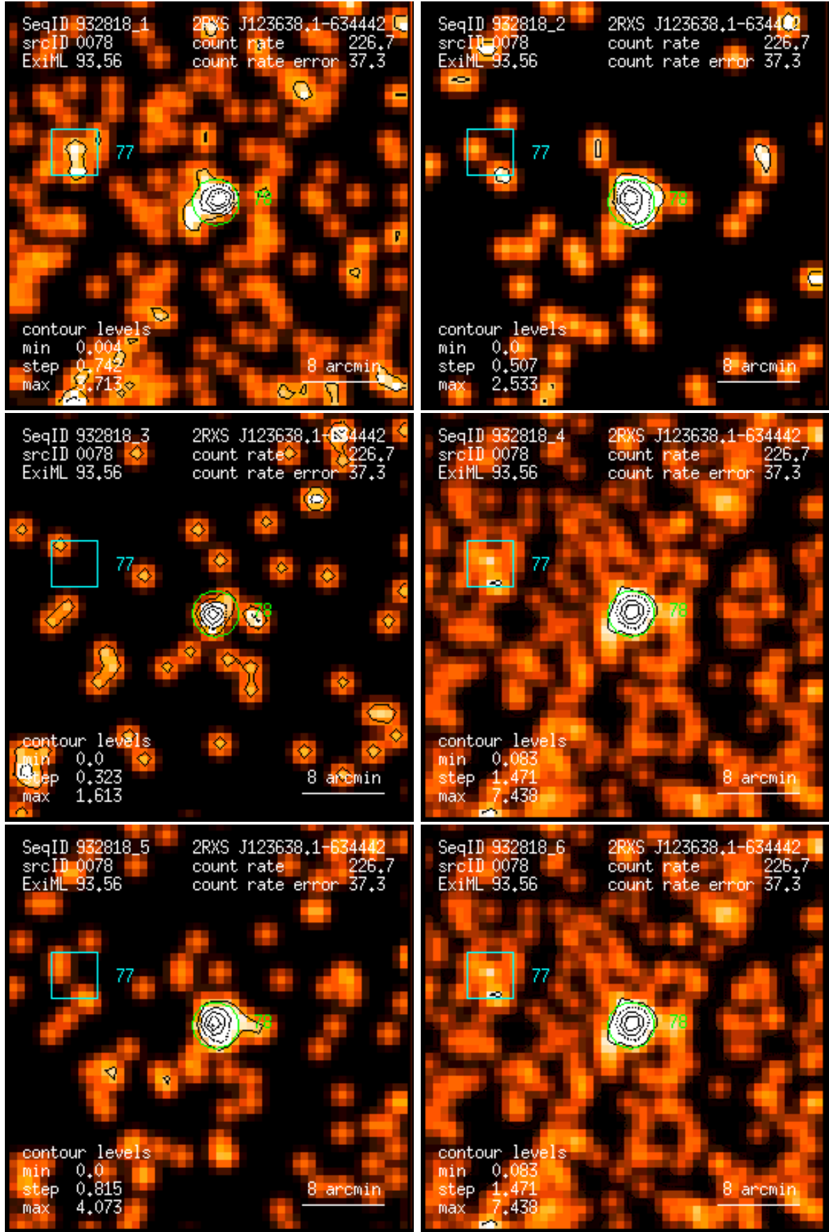
Figure 78: RASS 932818: detection 0078: band rate images, Gaussian filter: (1) PSPC channels 11 – 41, (2) 52 – 90, (3) 91 – 201, (4) 11 – 235, (5) 52 – 201, (6) 11 – 201. Broad band rates in counts/ks. Band rate contour levels in counts/ks/arcmin 2 .
