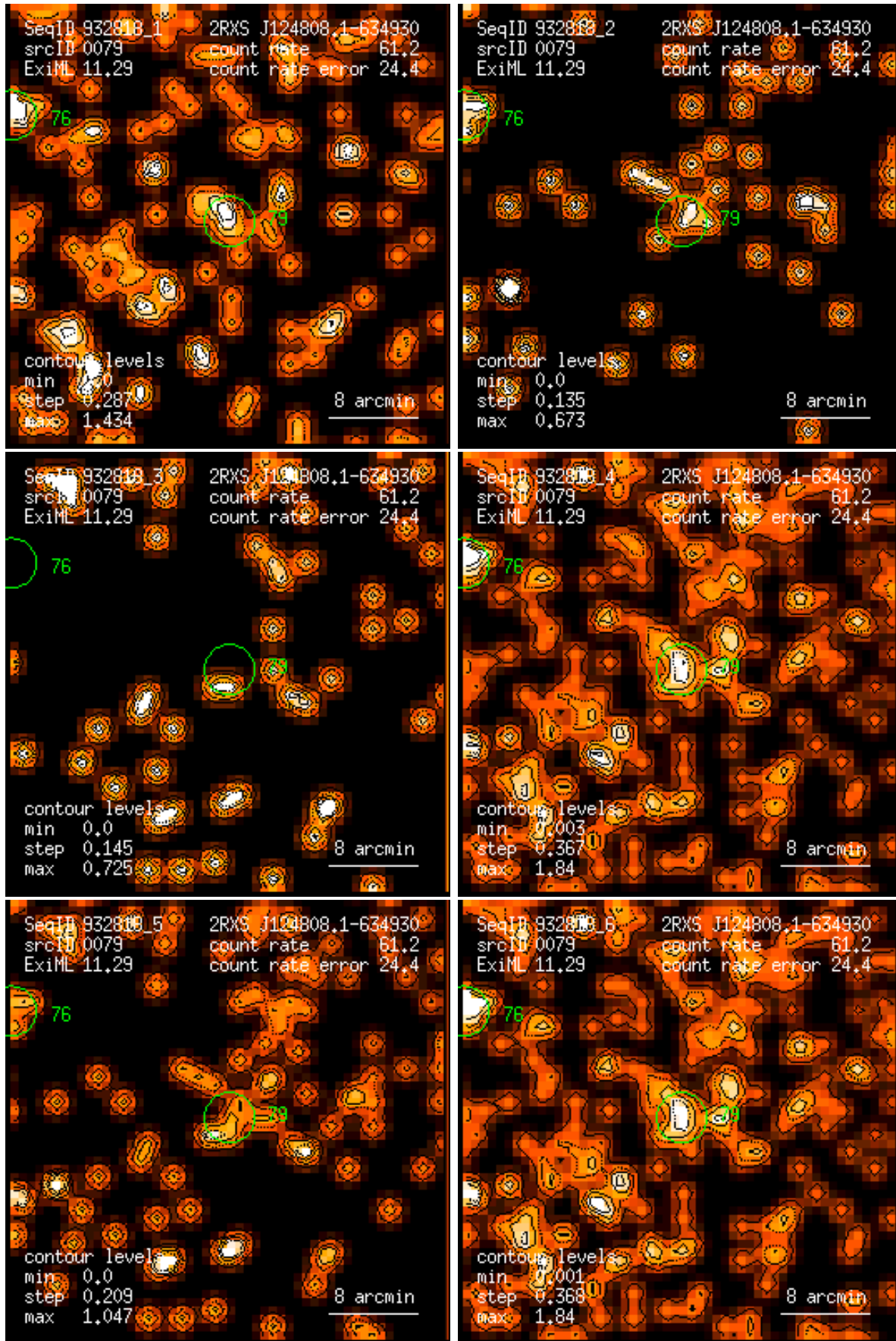
Figure 79: RASS 932818: detection 0079: band rate images, Gaussian filter: (1) PSPC channels 11 – 41, (2) 52 – 90, (3) 91 – 201, (4) 11 – 235, (5) 52 – 201, (6) 11 – 201. Broad band rates in counts/ks. Band rate contour levels in counts/ks/arcmin 2 .
