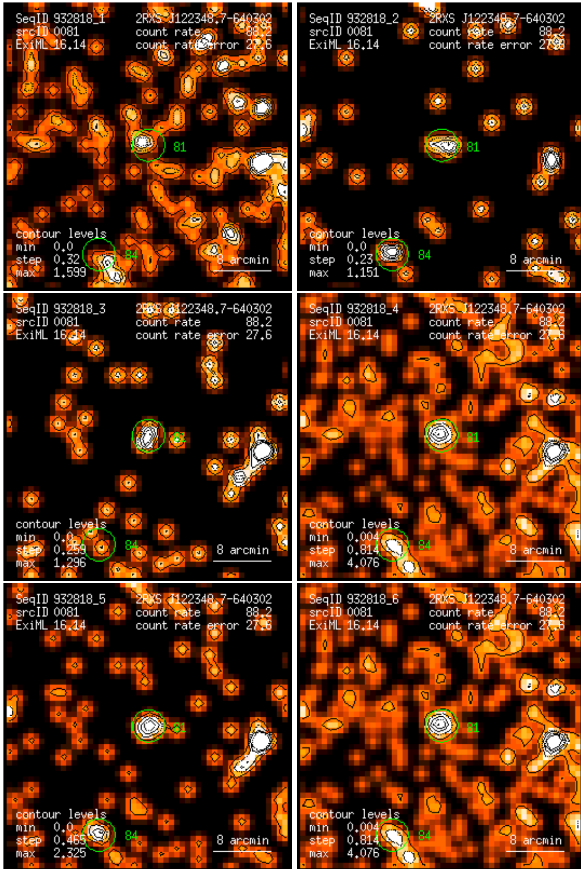
Figure 81: RASS 932818: detection 0081: band rate images, Gaussian filter: (1) PSPC channels 11 – 41, (2) 52 – 90, (3) 91 – 201, (4) 11 – 235, (5) 52 – 201, (6) 11 – 201. Broad band rates in counts/ks. Band rate contour levels in counts/ks/arcmin 2 .
