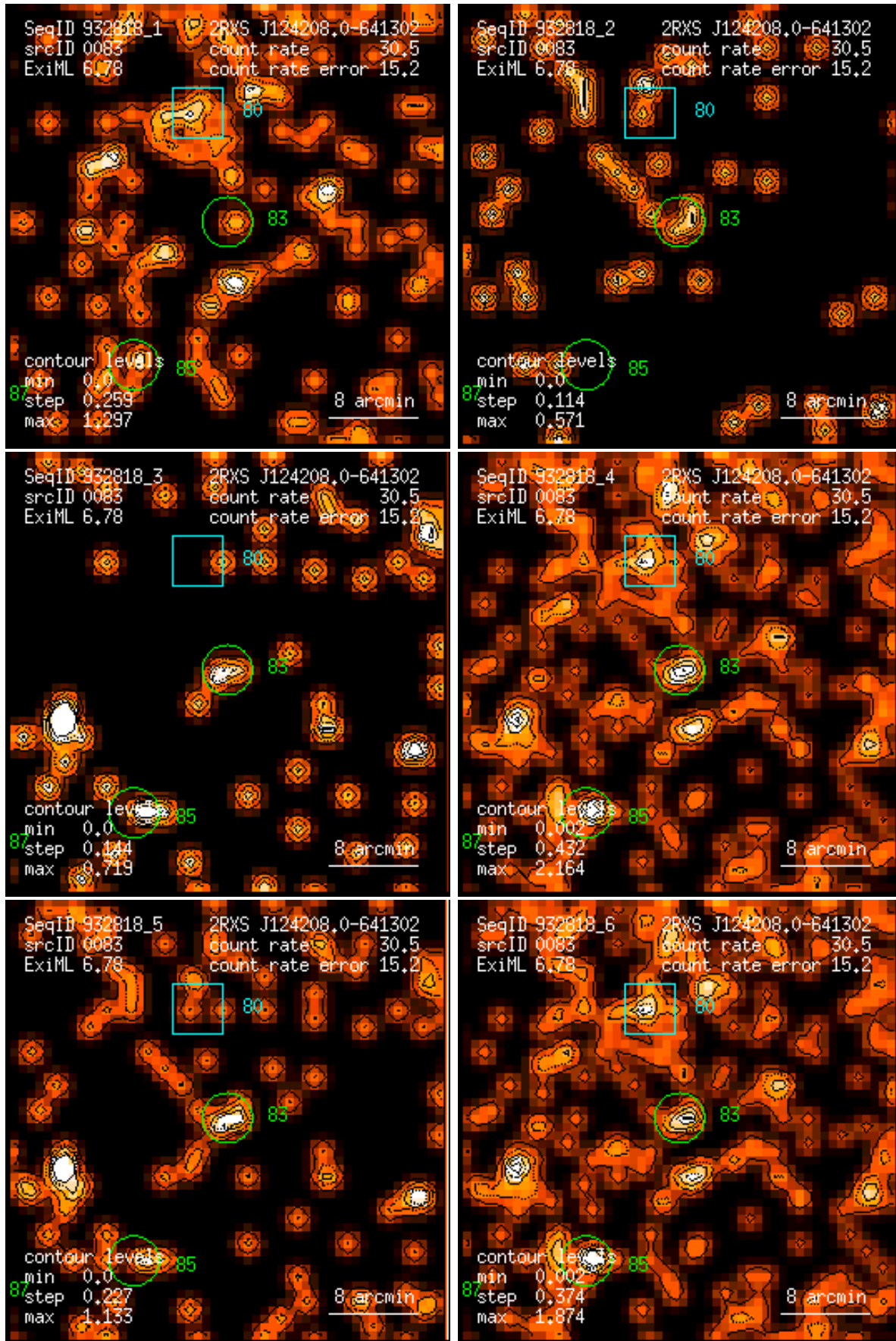
Figure 83: RASS 932818: detection 0083: band rate images, Gaussian filter: (1) PSPC channels 11 – 41, (2) 52 – 90, (3) 91 – 201, (4) 11 – 235, (5) 52 – 201, (6) 11 – 201. Broad band rates in counts/ks. Band rate contour levels in counts/ks/arcmin 2 .
