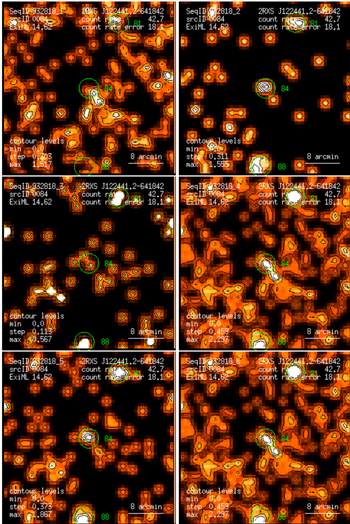
Figure 84: RASS 932818: detection 0084: band rate images, Gaussian filter: (1) PSPC channels 11 – 41, (2) 52 – 90, (3) 91 – 201, (4) 11 – 235, (5) 52 – 201, (6) 11 – 201. Broad band rates in counts/ks. Band rate contour levels in counts/ks/arcmin 2 .
