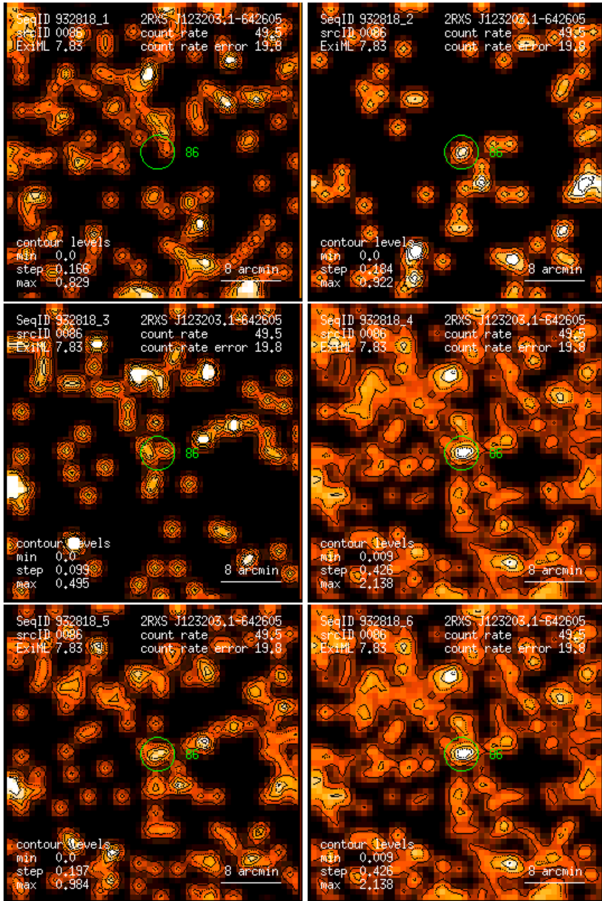
Figure 86: RASS 932818: detection 0086: band rate images, Gaussian filter: (1) PSPC channels 11 – 41, (2) 52 – 90, (3) 91 – 201, (4) 11 – 235, (5) 52 – 201, (6) 11 – 201. Broad band rates in counts/ks. Band rate contour levels in counts/ks/arcmin 2 .
