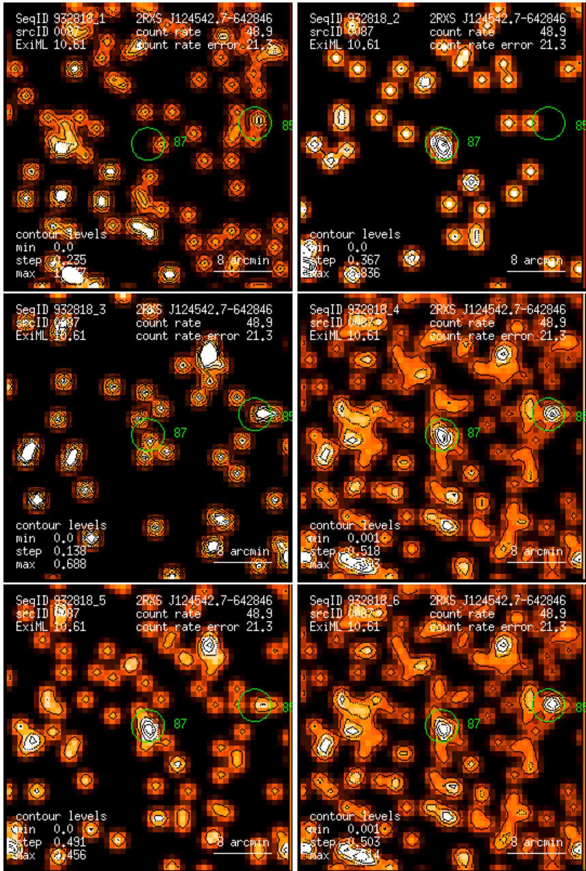
Figure 87: RASS 932818: detection 0087: band rate images, Gaussian filter: (1) PSPC channels 11 – 41, (2) 52 – 90, (3) 91 – 201, (4) 11 – 235, (5) 52 – 201, (6) 11 – 201. Broad band rates in counts/ks. Band rate contour levels in counts/ks/arcmin 2 .
