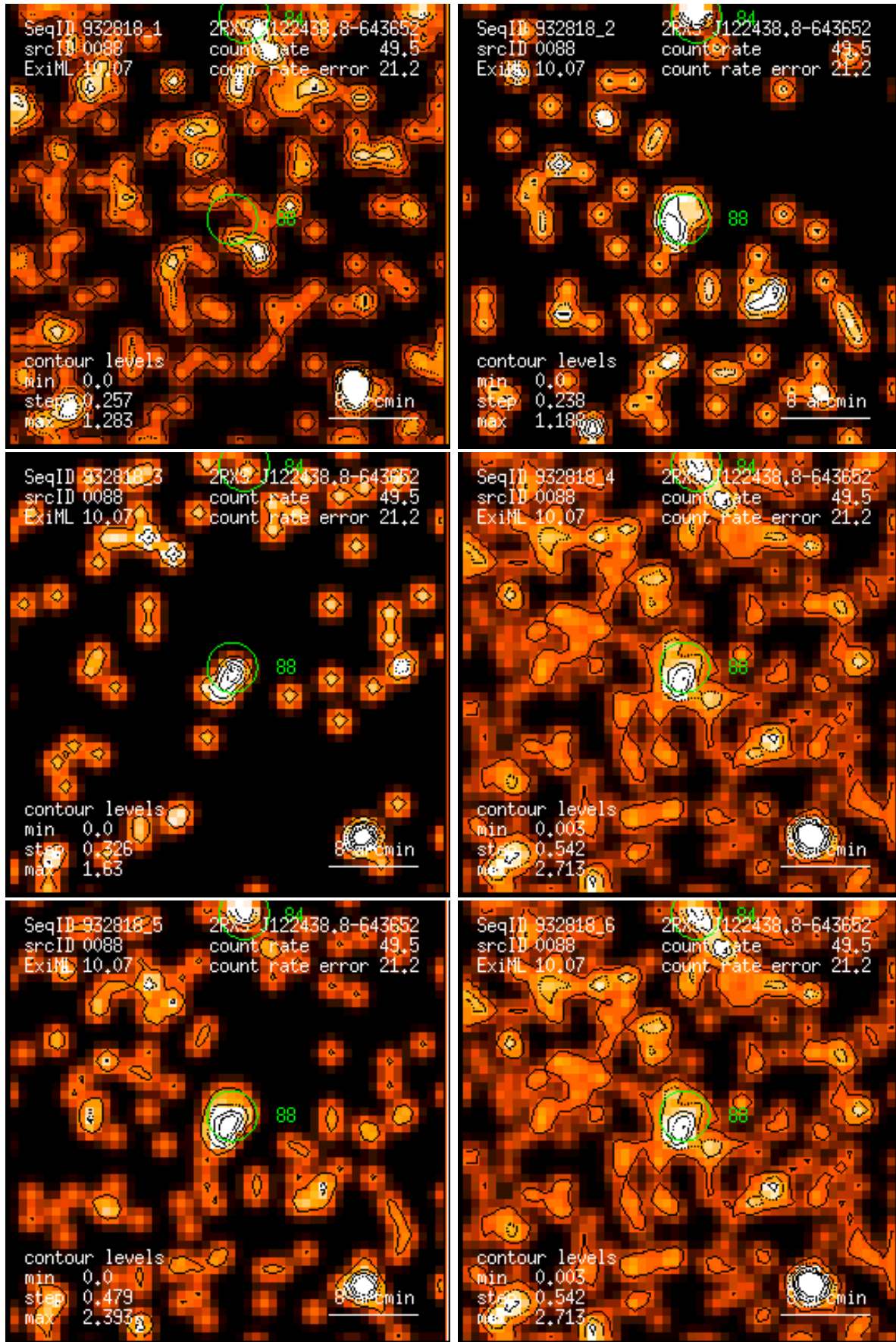
Figure 88: RASS 932818: detection 0088: band rate images, Gaussian filter: (1) PSPC channels 11 – 41, (2) 52 – 90, (3) 91 – 201, (4) 11 – 235, (5) 52 – 201, (6) 11 – 201. Broad band rates in counts/ks. Band rate contour levels in counts/ks/arcmin 2 .
