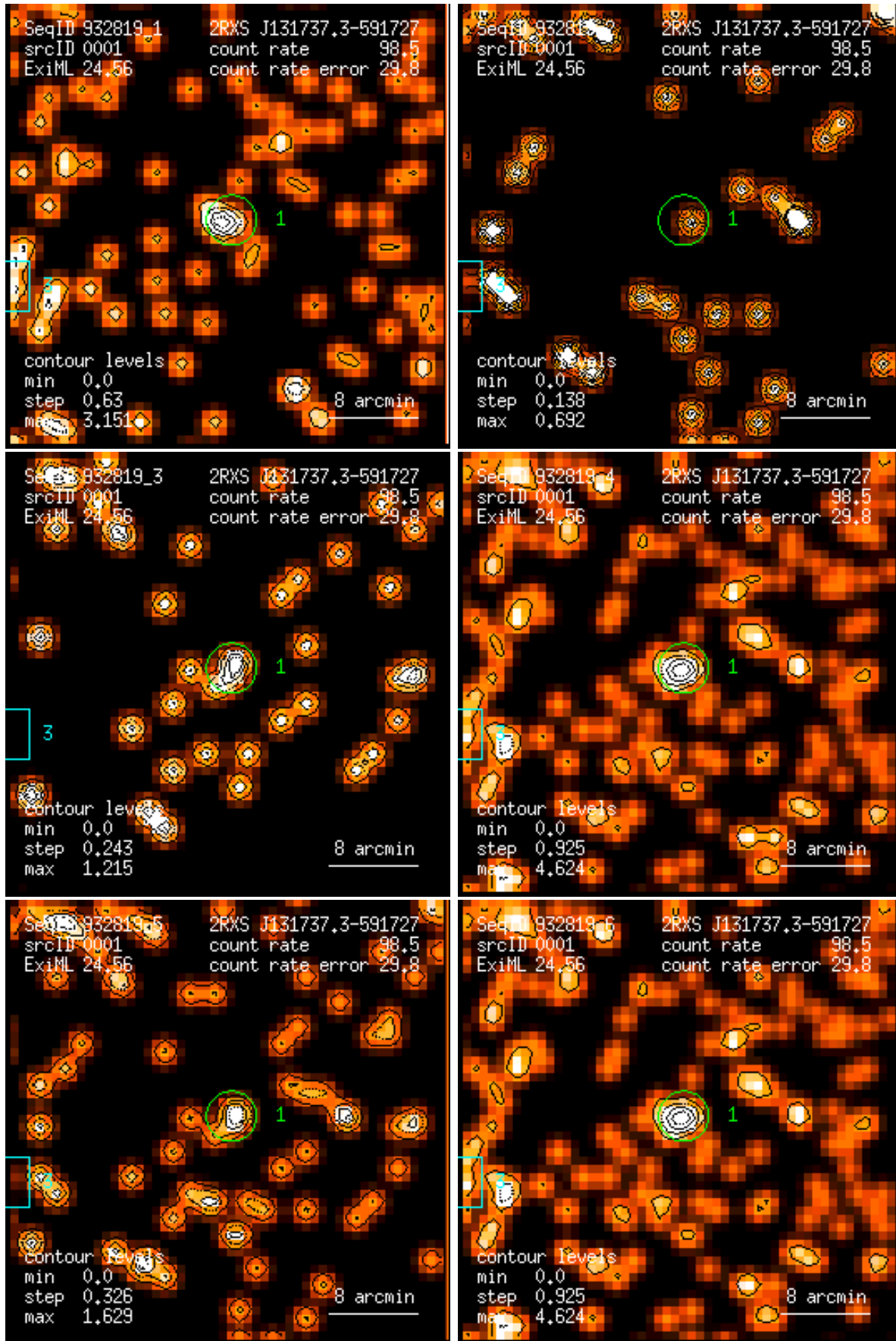
Figure 1: RASS 932819: detection 0001: band rate images, Gaussian filter: (1) PSPC channels 11 – 41, (2) 52 – 90, (3) 91 – 201, (4) 11 – 235, (5) 52 – 201, (6) 11 – 201. Broad band rates in counts/ks. Band rate contour levels in counts/ks/arcmin 2 .
