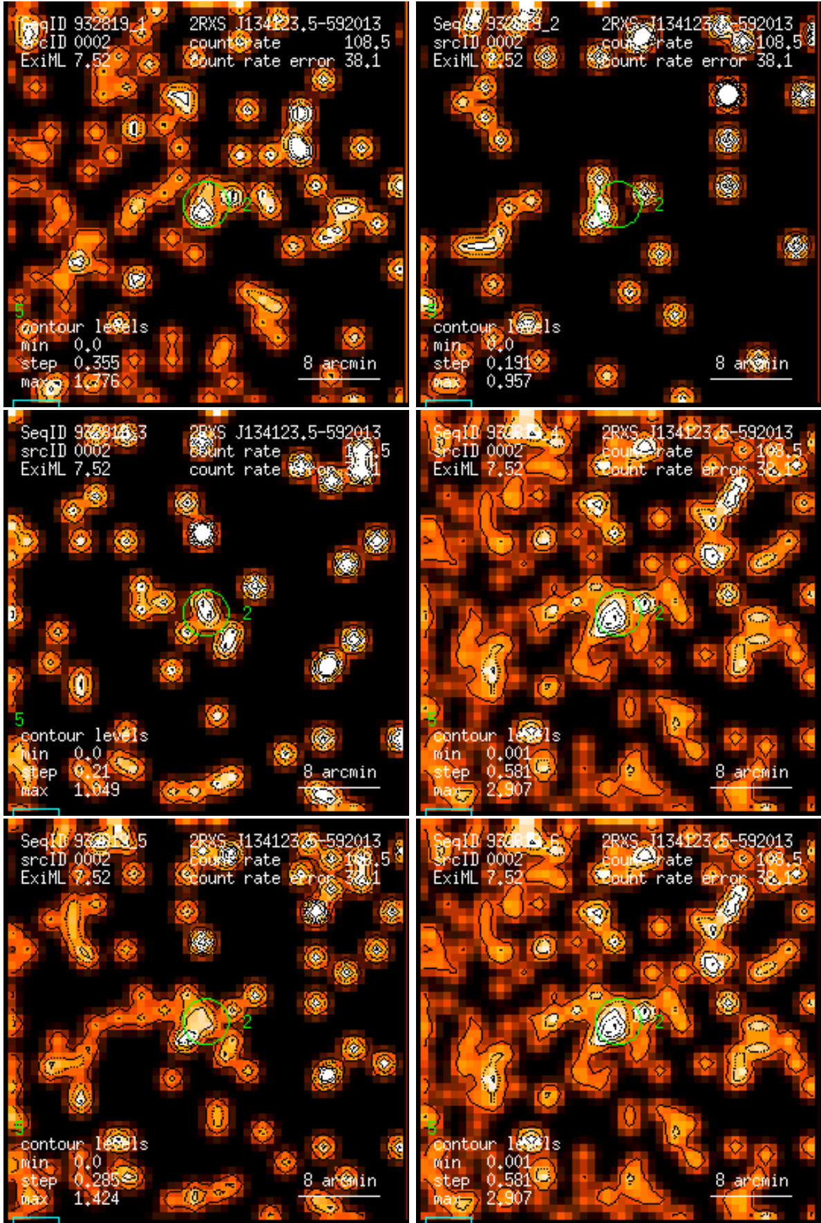
Figure 2: RASS 932819: detection 0002: band rate images, Gaussian filter: (1) PSPC channels 11 – 41, (2) 52 – 90, (3) 91 – 201, (4) 11 – 235, (5) 52 – 201, (6) 11 – 201. Broad band rates in counts/ks. Band rate contour levels in counts/ks/arcmin 2 .
