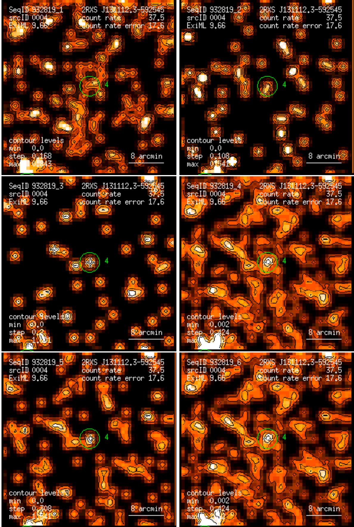
Figure 4: RASS 932819: detection 0004: band rate images, Gaussian filter: (1) PSPC channels 11 – 41, (2) 52 – 90, (3) 91 – 201, (4) 11 – 235, (5) 52 – 201, (6) 11 – 201. Broad band rates in counts/ks. Band rate contour levels in counts/ks/arcmin 2 .
