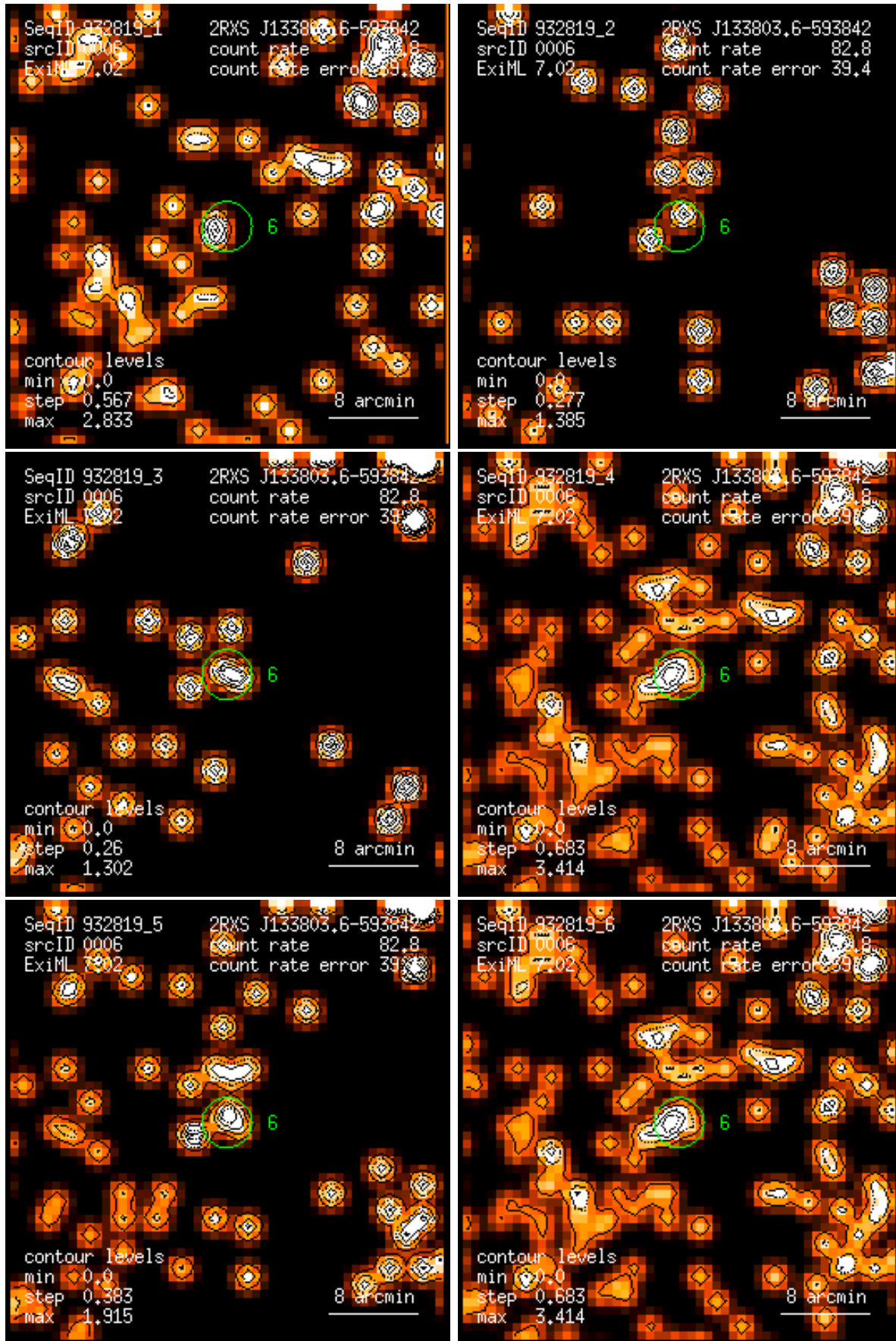
Figure 6: RASS 932819: detection 0006: band rate images, Gaussian filter: (1) PSPC channels 11 – 41, (2) 52 – 90, (3) 91 – 201, (4) 11 – 235, (5) 52 – 201, (6) 11 – 201. Broad band rates in counts/ks. Band rate contour levels in counts/ks/arcmin 2 .
