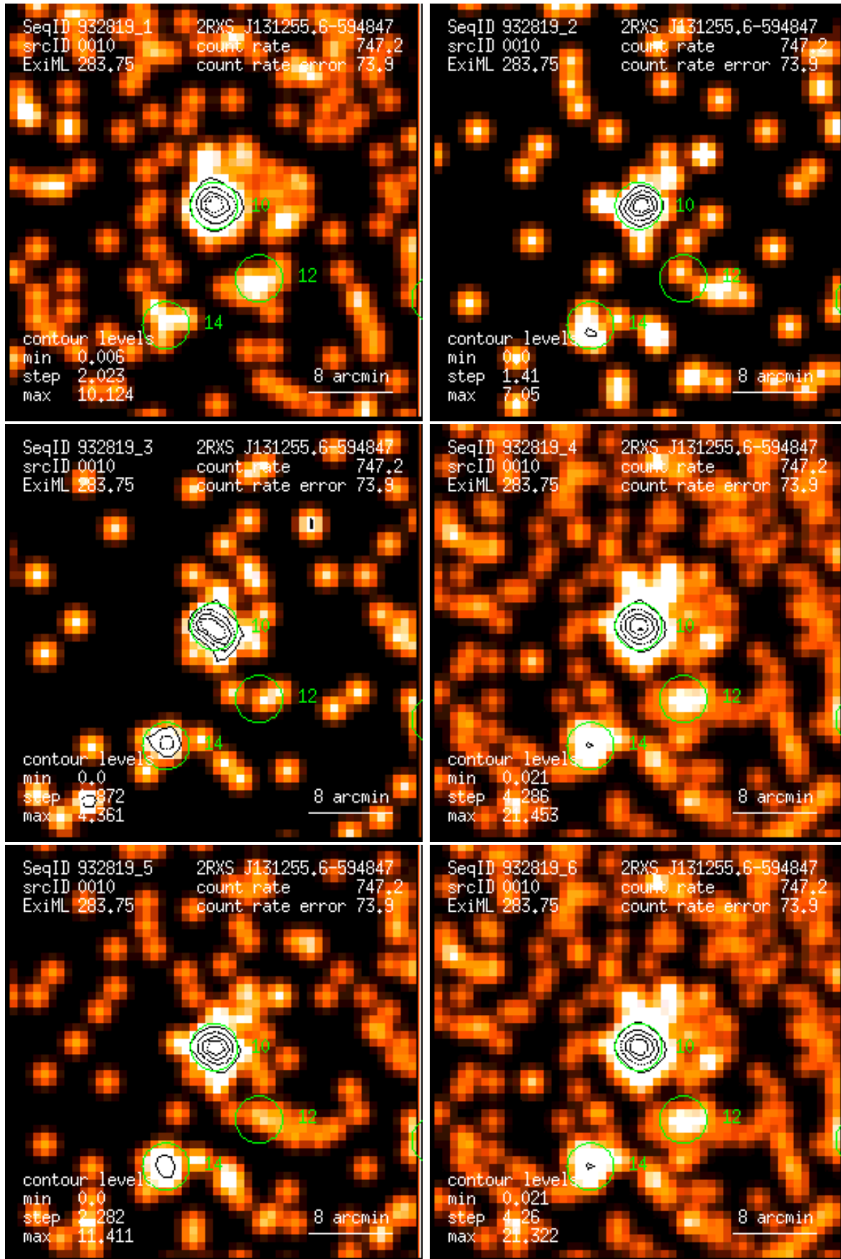
Figure 10: RASS 932819: detection 0010: band rate images, Gaussian filter: (1) PSPC channels 11 – 41, (2) 52 – 90, (3) 91 – 201, (4) 11 – 235, (5) 52 – 201, (6) 11 – 201. Broad band rates in counts/ks. Band rate contour levels in counts/ks/arcmin 2 .
