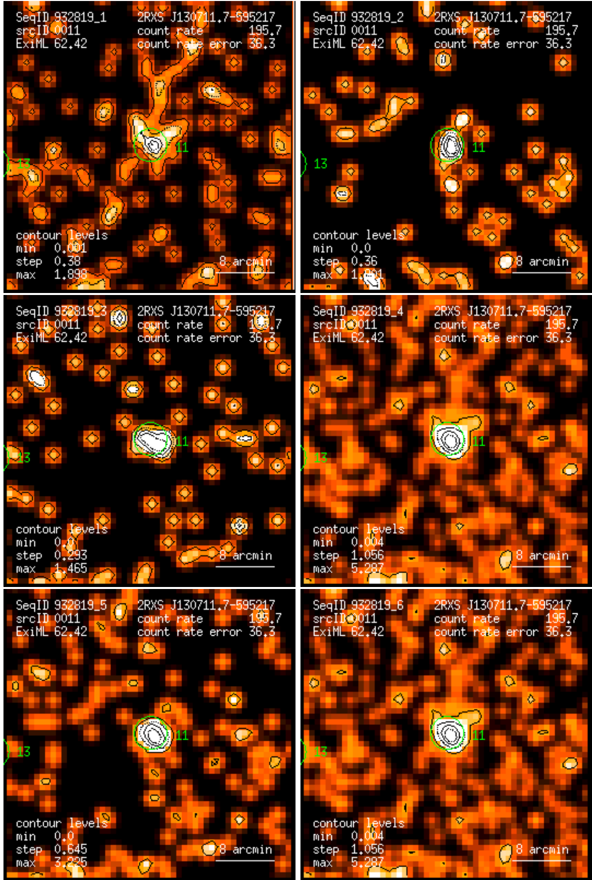
Figure 11: RASS 932819: detection 0011: band rate images, Gaussian filter: (1) PSPC channels 11 – 41, (2) 52 – 90, (3) 91 – 201, (4) 11 – 235, (5) 52 – 201, (6) 11 – 201. Broad band rates in counts/ks. Band rate contour levels in counts/ks/arcmin 2 .
