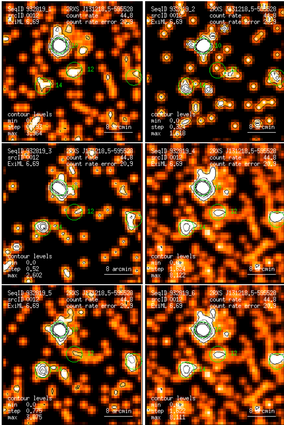
Figure 12: RASS 932819: detection 0012: band rate images, Gaussian filter: (1) PSPC channels 11 – 41, (2) 52 – 90, (3) 91 – 201, (4) 11 – 235, (5) 52 – 201, (6) 11 – 201. Broad band rates in counts/ks. Band rate contour levels in counts/ks/arcmin 2 .
