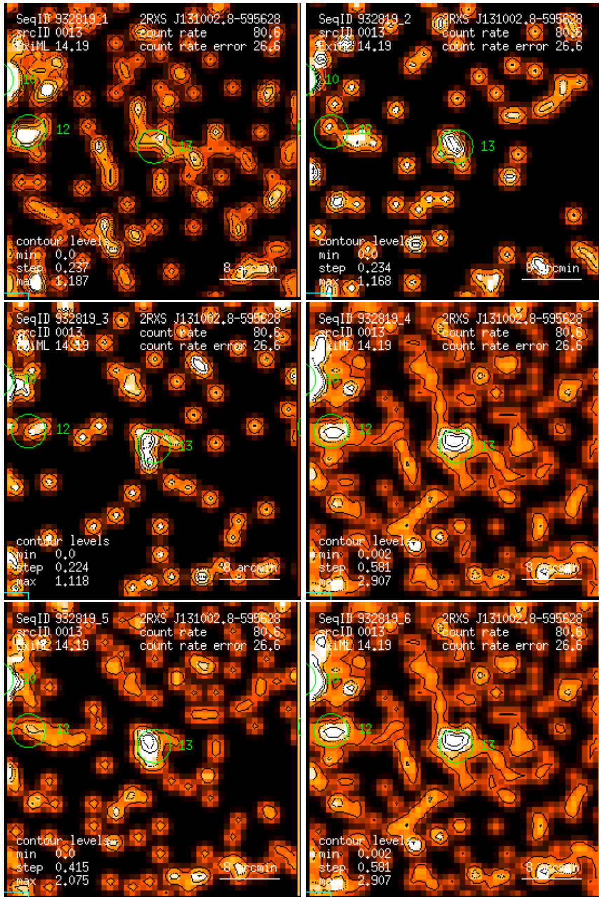
Figure 13: RASS 932819: detection 0013: band rate images, Gaussian filter: (1) PSPC channels 11 – 41, (2) 52 – 90, (3) 91 – 201, (4) 11 – 235, (5) 52 – 201, (6) 11 – 201. Broad band rates in counts/ks. Band rate contour levels in counts/ks/arcmin 2 .
