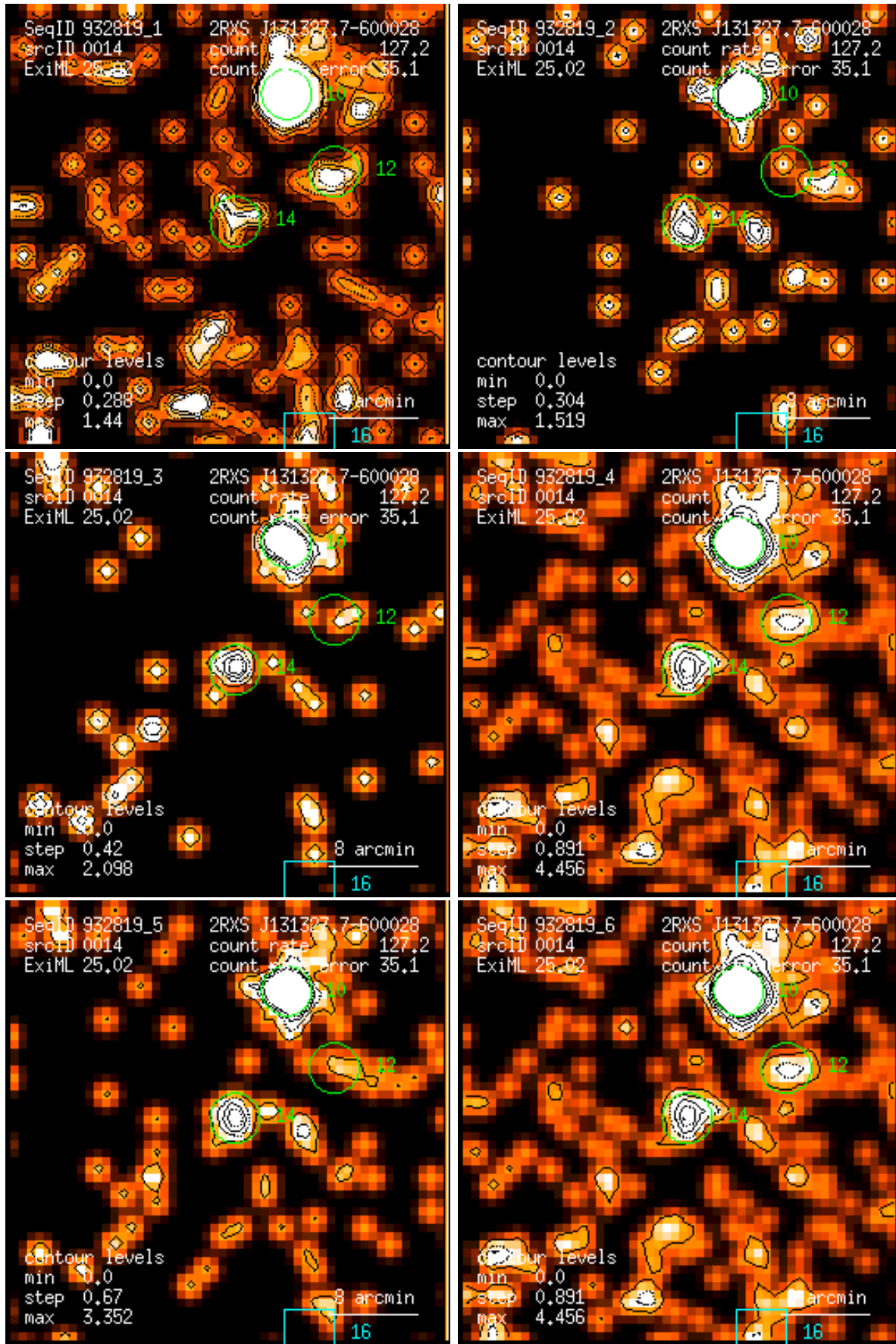
Figure 14: RASS 932819: detection 0014: band rate images, Gaussian filter: (1) PSPC channels 11 – 41, (2) 52 – 90, (3) 91 – 201, (4) 11 – 235, (5) 52 – 201, (6) 11 – 201. Broad band rates in counts/ks. Band rate contour levels in counts/ks/arcmin 2 .
