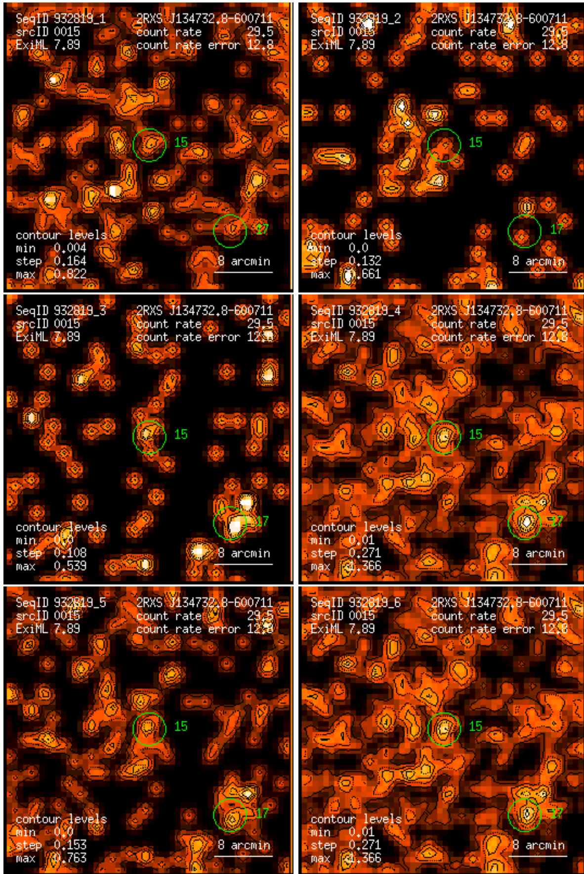
Figure 15: RASS 932819: detection 0015: band rate images, Gaussian filter: (1) PSPC channels 11 – 41, (2) 52 – 90, (3) 91 – 201, (4) 11 – 235, (5) 52 – 201, (6) 11 – 201. Broad band rates in counts/ks. Band rate contour levels in counts/ks/arcmin 2 .
