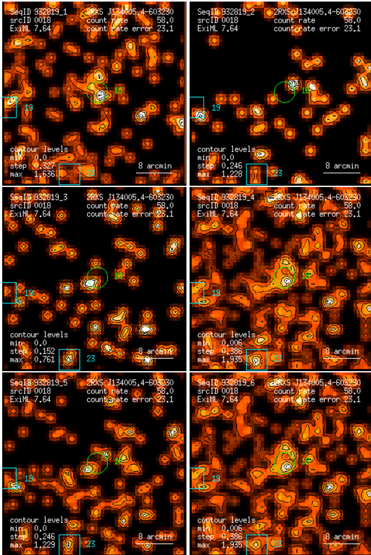
Figure 18: RASS 932819: detection 0018: band rate images, Gaussian filter: (1) PSPC channels 11 – 41, (2) 52 – 90, (3) 91 – 201, (4) 11 – 235, (5) 52 – 201, (6) 11 – 201. Broad band rates in counts/ks. Band rate contour levels in counts/ks/arcmin 2 .
