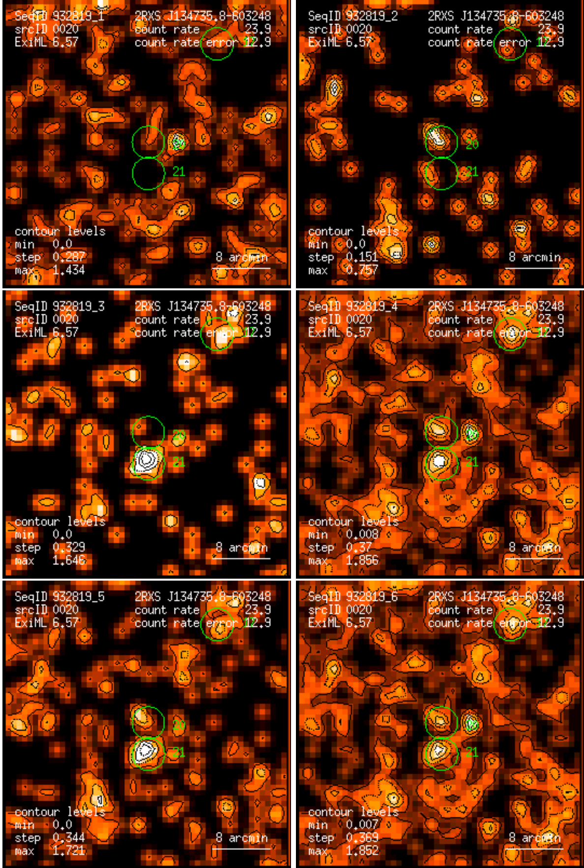
Figure 20: RASS 932819: detection 0020: band rate images, Gaussian filter: (1) PSPC channels 11 – 41, (2) 52 – 90, (3) 91 – 201, (4) 11 – 235, (5) 52 – 201, (6) 11 – 201. Broad band rates in counts/ks. Band rate contour levels in counts/ks/arcmin 2 .
