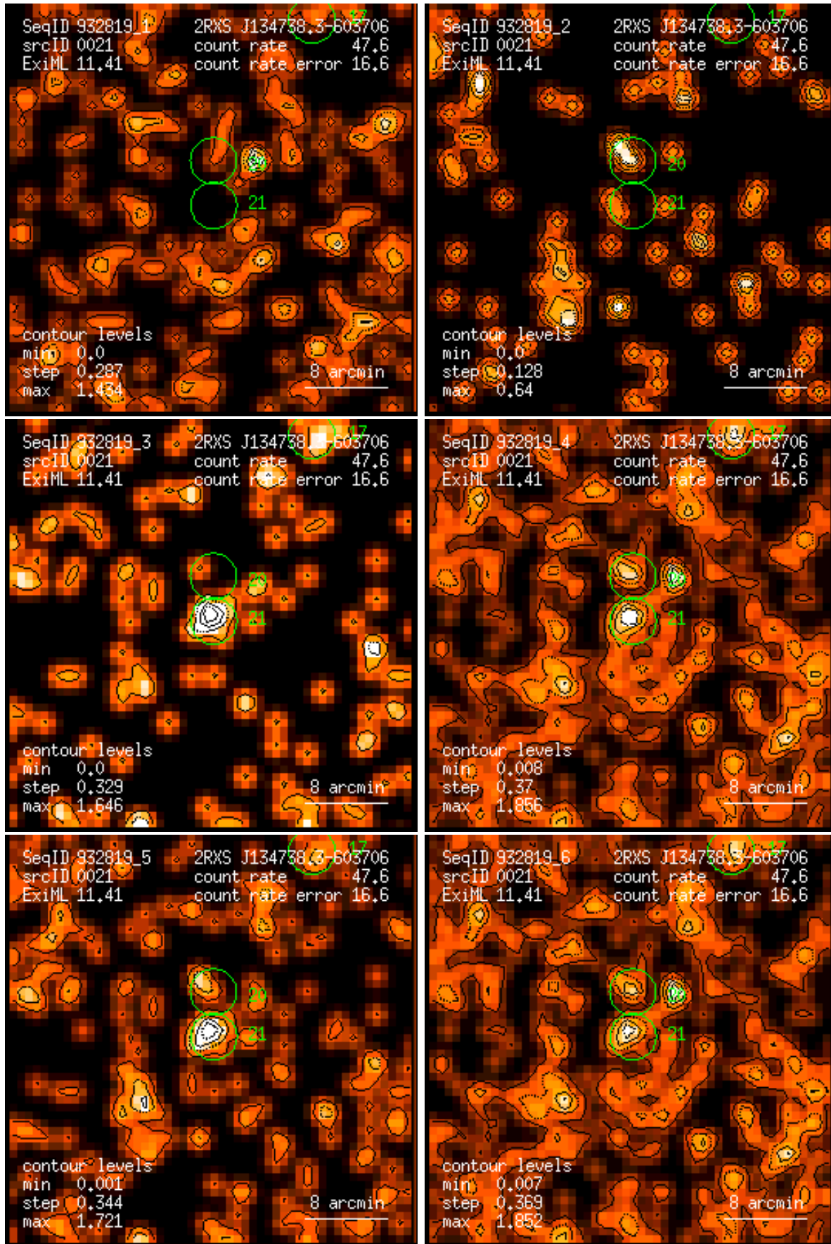
Figure 21: RASS 932819: detection 0021: band rate images, Gaussian filter: (1) PSPC channels 11 – 41, (2) 52 – 90, (3) 91 – 201, (4) 11 – 235, (5) 52 – 201, (6) 11 – 201. Broad band rates in counts/ks. Band rate contour levels in counts/ks/arcmin 2 .
