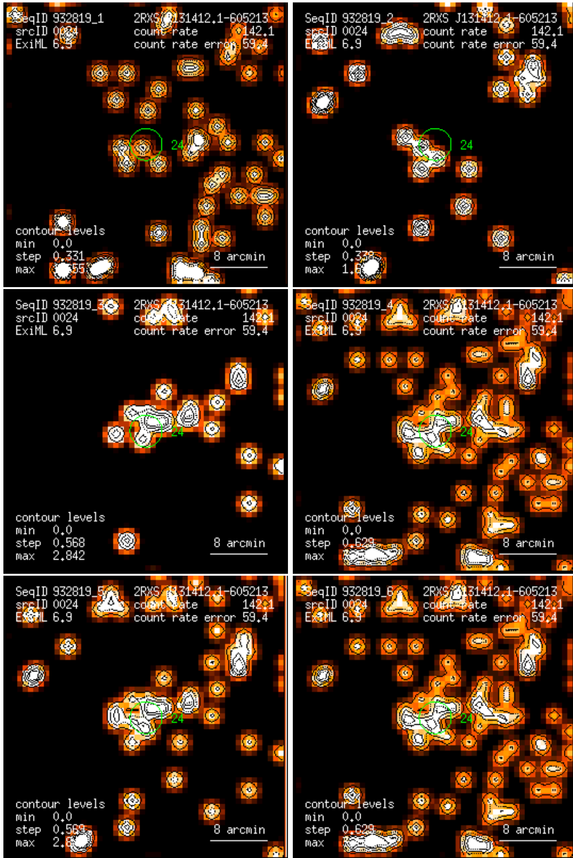
Figure 24: RASS 932819: detection 0024: band rate images, Gaussian filter: (1) PSPC channels 11 – 41, (2) 52 – 90, (3) 91 – 201, (4) 11 – 235, (5) 52 – 201, (6) 11 – 201. Broad band rates in counts/ks. Band rate contour levels in counts/ks/arcmin 2 .
