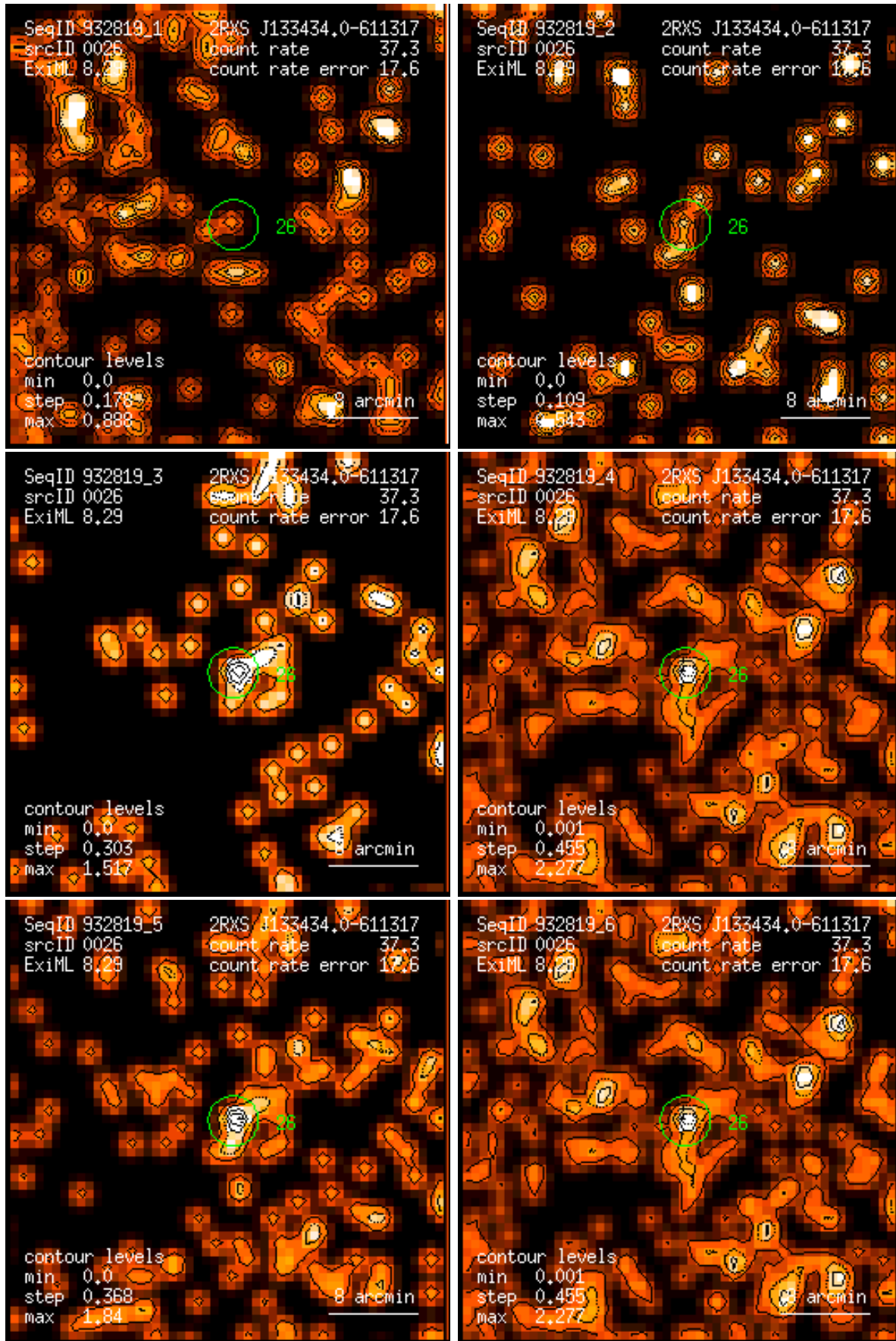
Figure 26: RASS 932819: detection 0026: band rate images, Gaussian filter: (1) PSPC channels 11 – 41, (2) 52 – 90, (3) 91 – 201, (4) 11 – 235, (5) 52 – 201, (6) 11 – 201. Broad band rates in counts/ks. Band rate contour levels in counts/ks/arcmin 2 .
