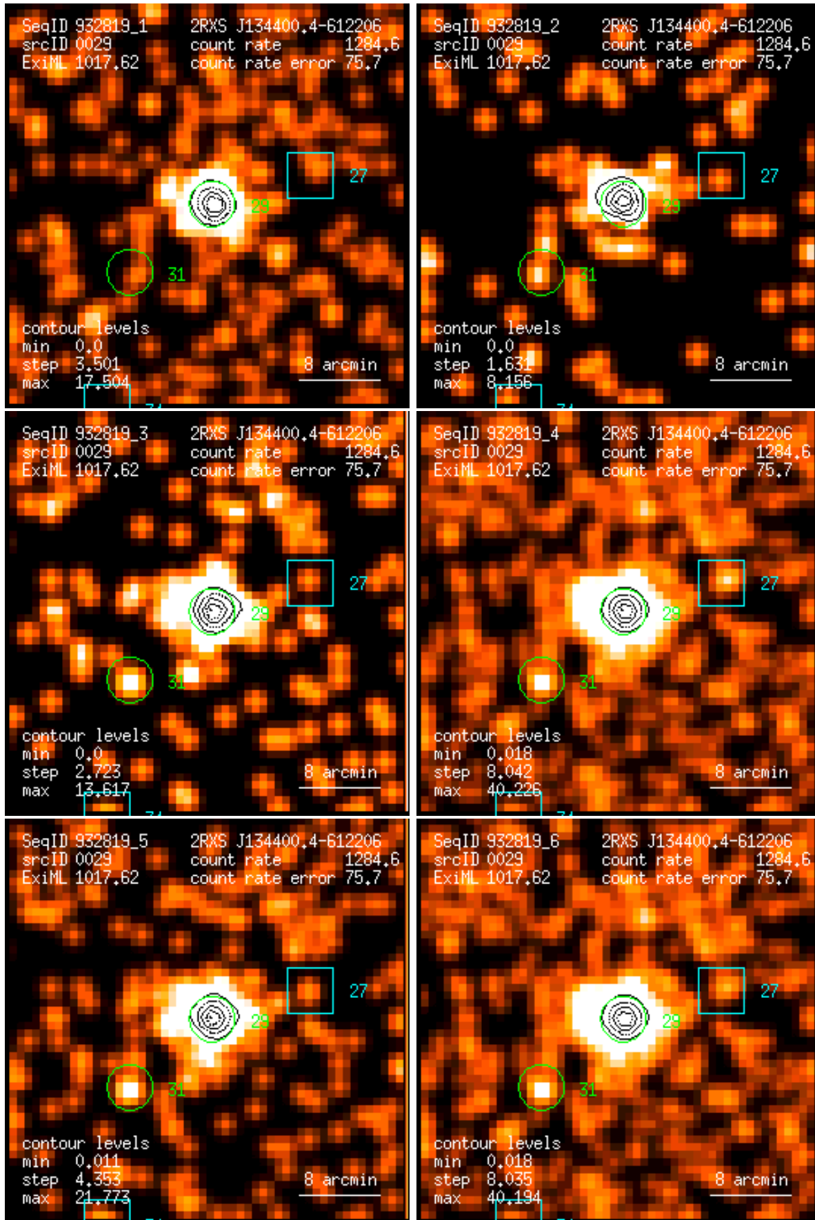
Figure 29: RASS 932819: detection 0029: band rate images, Gaussian filter: (1) PSPC channels 11 – 41, (2) 52 – 90, (3) 91 – 201, (4) 11 – 235, (5) 52 – 201, (6) 11 – 201. Broad band rates in counts/ks. Band rate contour levels in counts/ks/arcmin 2 .
