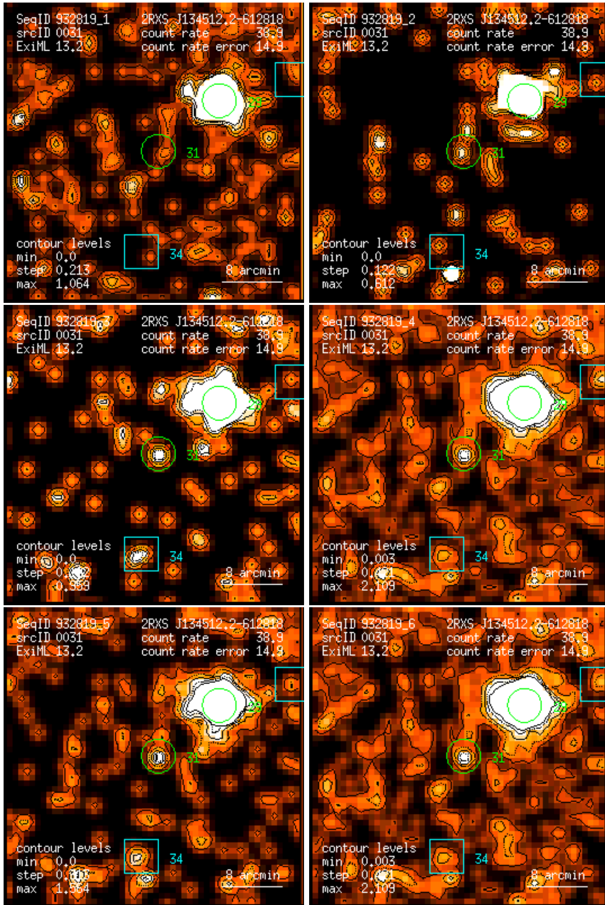
Figure 31: RASS 932819: detection 0031: band rate images, Gaussian filter: (1) PSPC channels 11 – 41, (2) 52 – 90, (3) 91 – 201, (4) 11 – 235, (5) 52 – 201, (6) 11 – 201. Broad band rates in counts/ks. Band rate contour levels in counts/ks/arcmin 2 .
