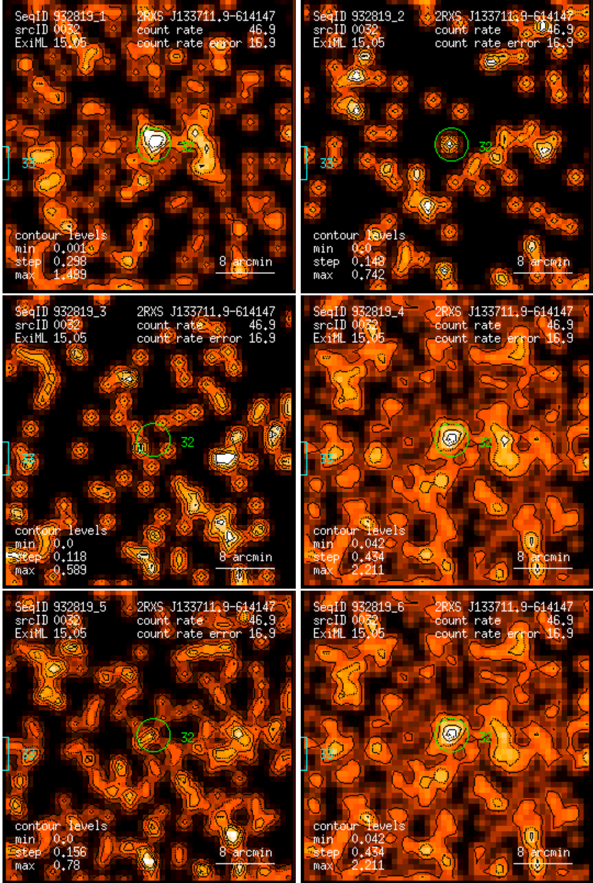
Figure 32: RASS 932819: detection 0032: band rate images, Gaussian filter: (1) PSPC channels 11 – 41, (2) 52 – 90, (3) 91 – 201, (4) 11 – 235, (5) 52 – 201, (6) 11 – 201. Broad band rates in counts/ks. Band rate contour levels in counts/ks/arcmin 2 .
