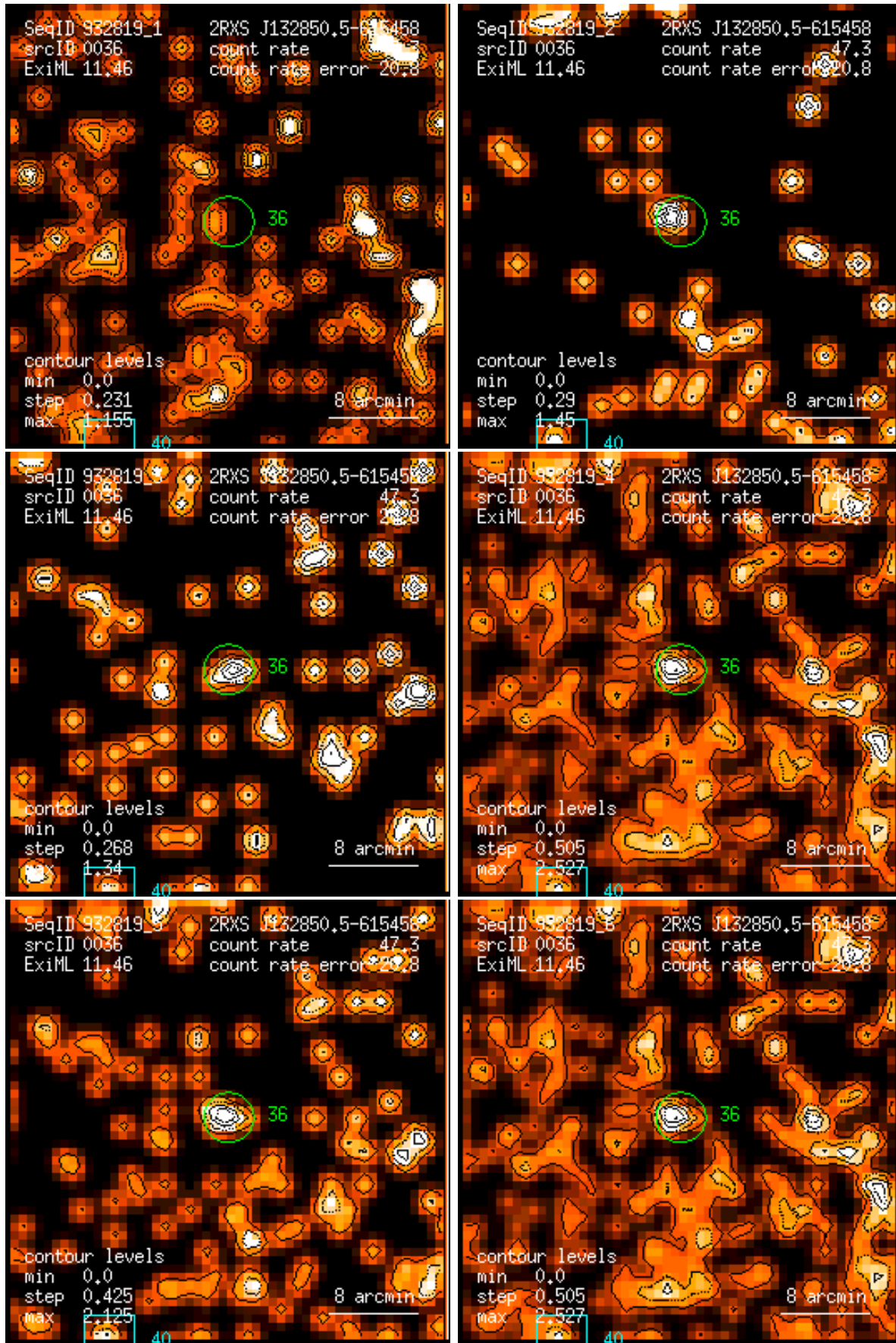
Figure 36: RASS 932819: detection 0036: band rate images, Gaussian filter: (1) PSPC channels 11 – 41, (2) 52 – 90, (3) 91 – 201, (4) 11 – 235, (5) 52 – 201, (6) 11 – 201. Broad band rates in counts/ks. Band rate contour levels in counts/ks/arcmin 2 .
