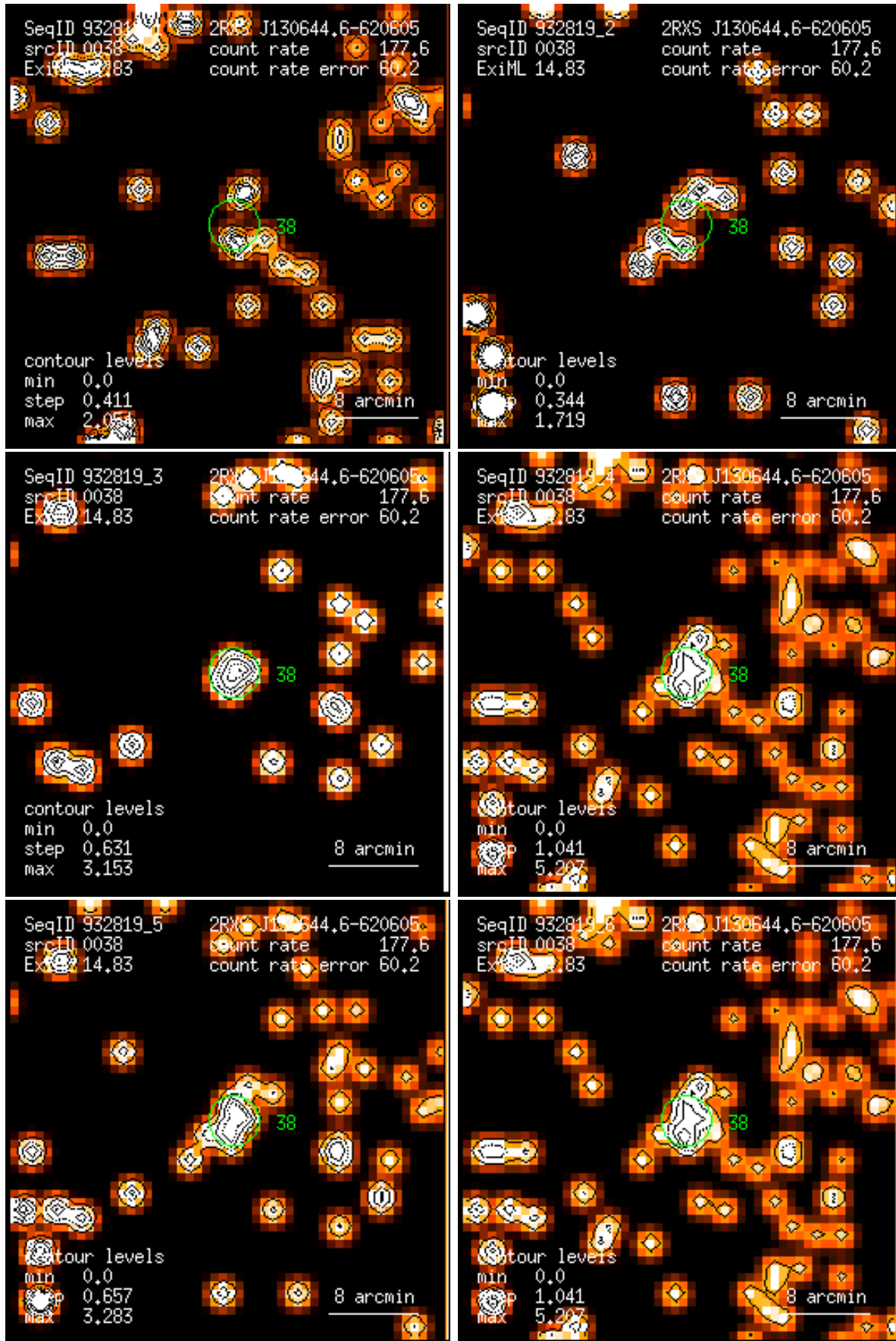
Figure 38: RASS 932819: detection 0038: band rate images, Gaussian filter: (1) PSPC channels 11 – 41, (2) 52 – 90, (3) 91 – 201, (4) 11 – 235, (5) 52 – 201, (6) 11 – 201. Broad band rates in counts/ks. Band rate contour levels in counts/ks/arcmin 2 .
