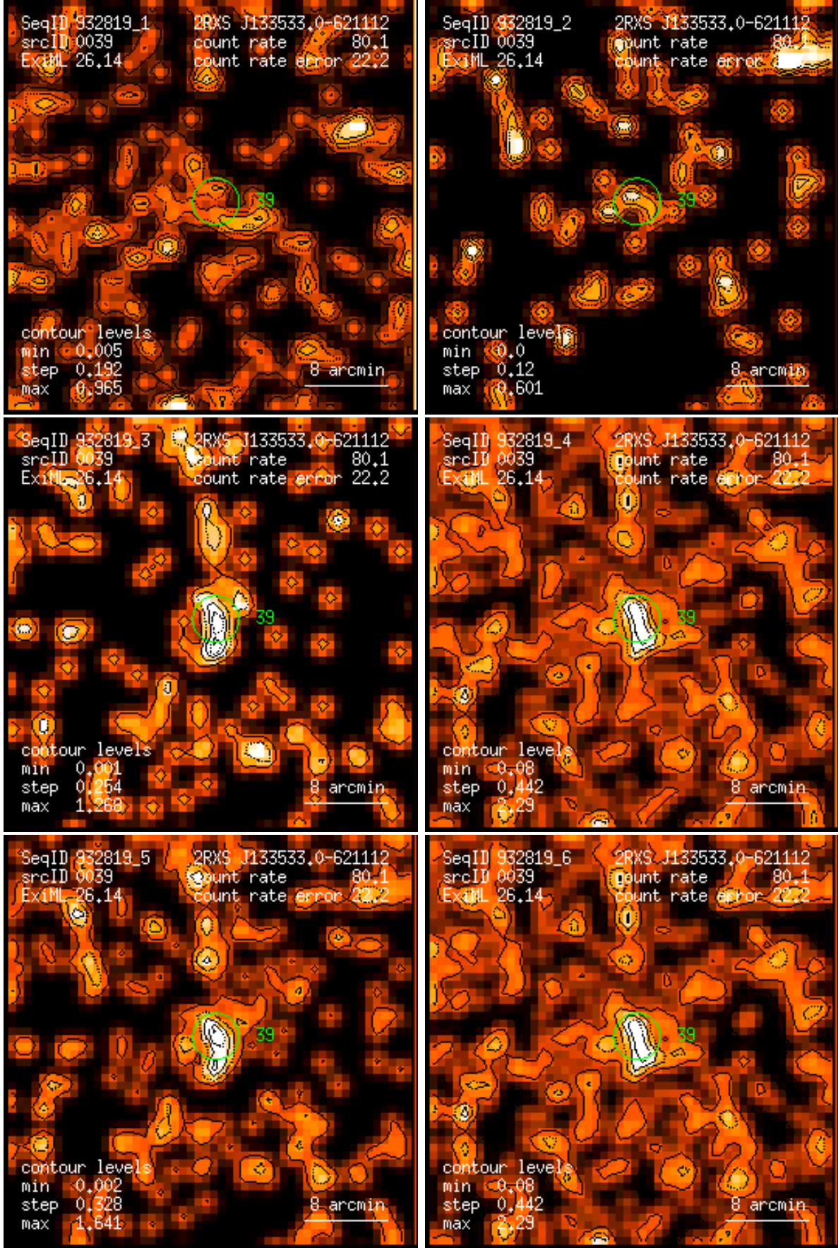
Figure 39: RASS 932819: detection 0039: band rate images, Gaussian filter: (1) PSPC channels 11 – 41, (2) 52 – 90, (3) 91 – 201, (4) 11 – 235, (5) 52 – 201, (6) 11 – 201. Broad band rates in counts/ks. Band rate contour levels in counts/ks/arcmin 2 .
