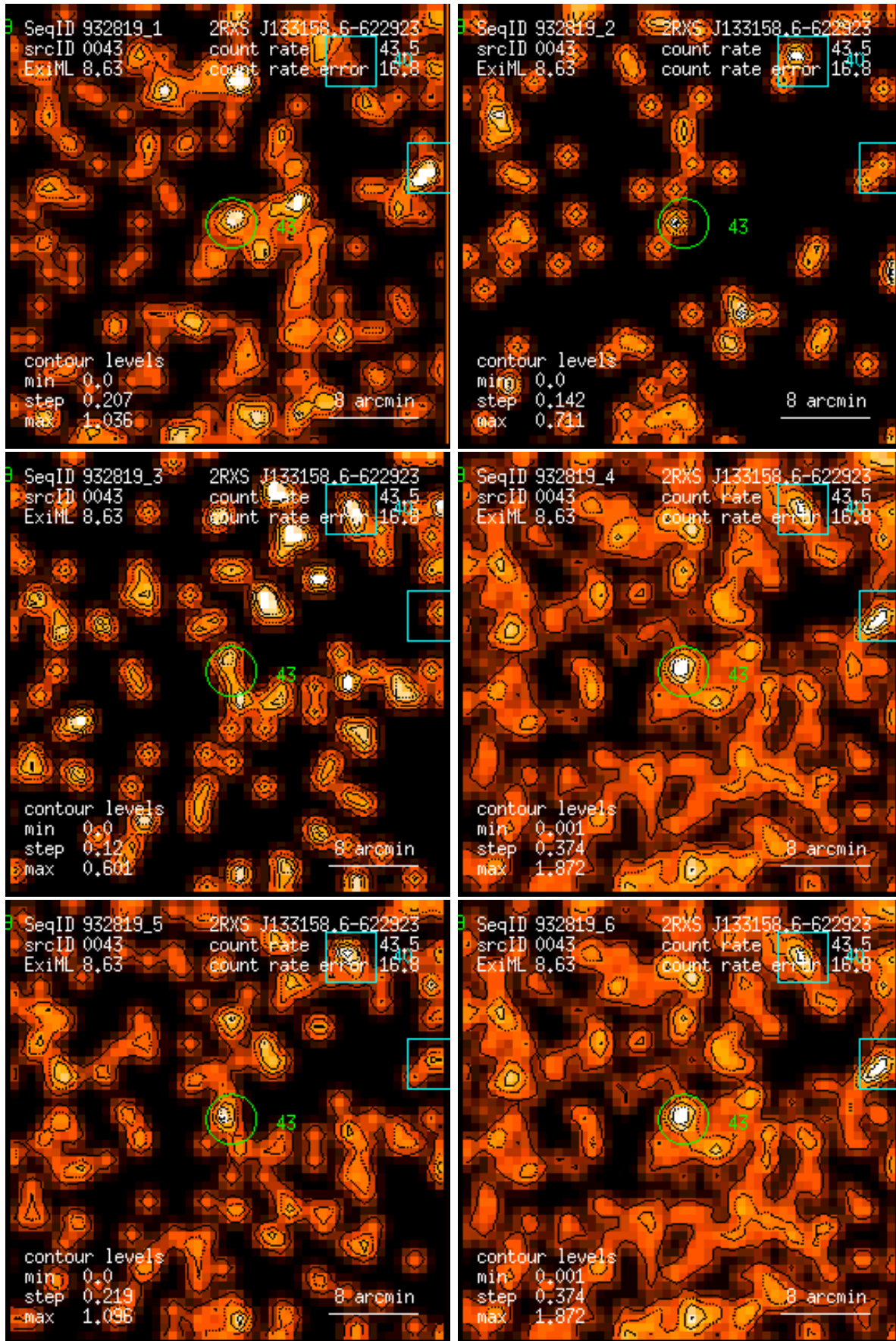
Figure 43: RASS 932819: detection 0043: band rate images, Gaussian filter: (1) PSPC channels 11 – 41, (2) 52 – 90, (3) 91 – 201, (4) 11 – 235, (5) 52 – 201, (6) 11 – 201. Broad band rates in counts/ks. Band rate contour levels in counts/ks/arcmin 2 .
