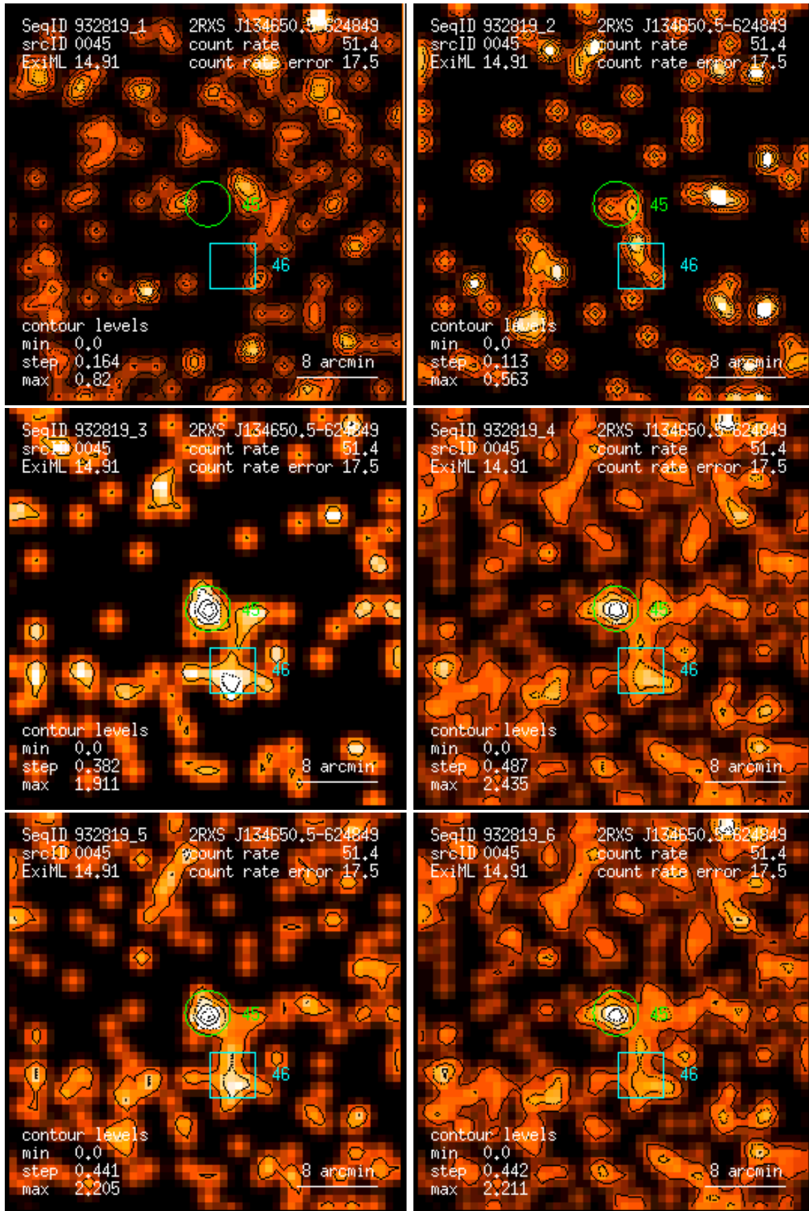
Figure 45: RASS 932819: detection 0045: band rate images, Gaussian filter: (1) PSPC channels 11 – 41, (2) 52 – 90, (3) 91 – 201, (4) 11 – 235, (5) 52 – 201, (6) 11 – 201. Broad band rates in counts/ks. Band rate contour levels in counts/ks/arcmin 2 .
