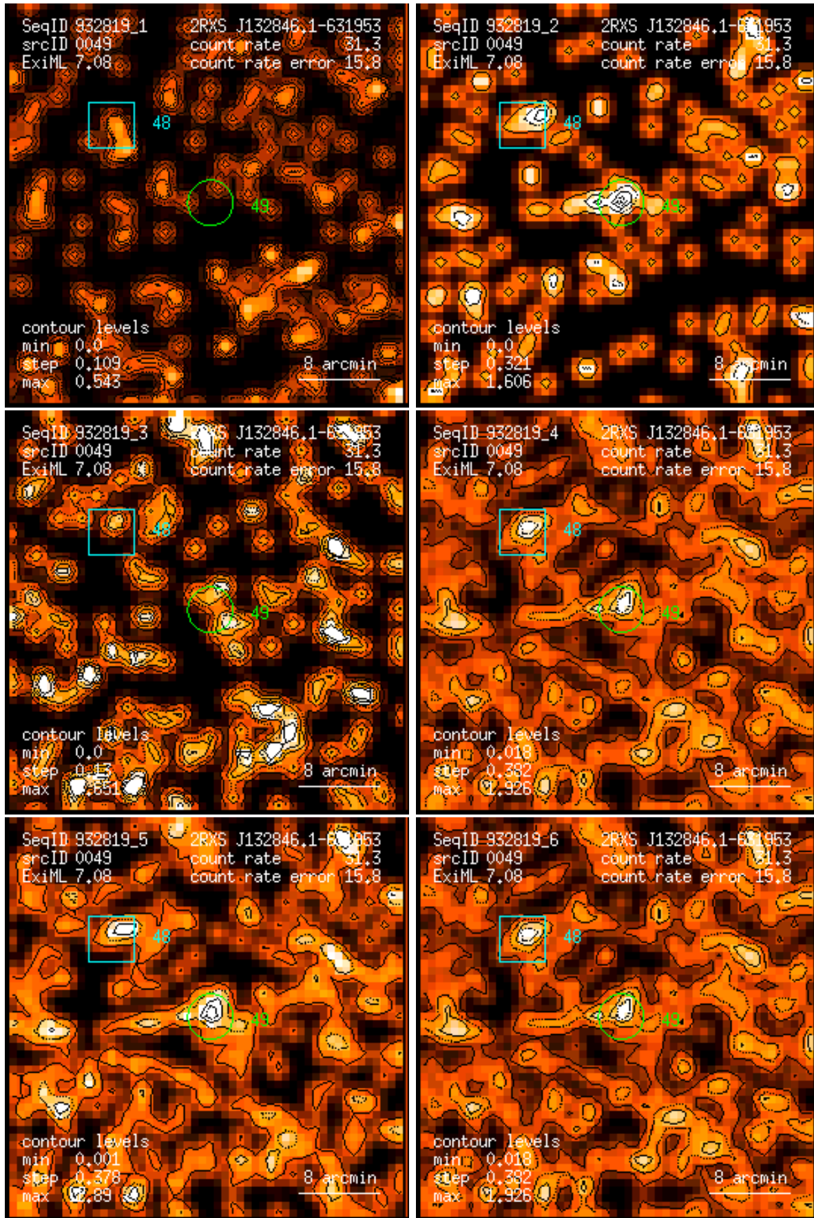
Figure 49: RASS 932819: detection 0049: band rate images, Gaussian filter: (1) PSPC channels 11 – 41, (2) 52 – 90, (3) 91 – 201, (4) 11 – 235, (5) 52 – 201, (6) 11 – 201. Broad band rates in counts/ks. Band rate contour levels in counts/ks/arcmin 2 .
