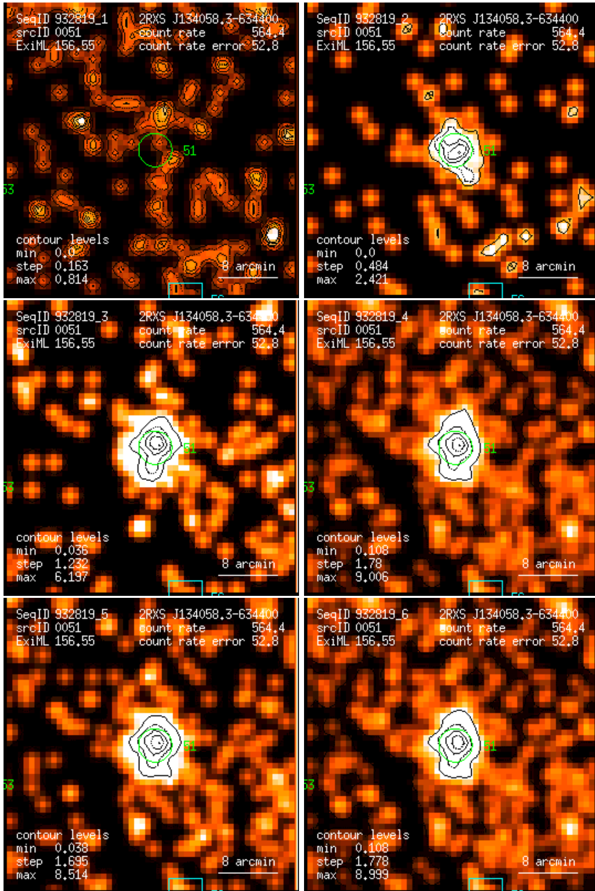
Figure 51: RASS 932819: detection 0051: band rate images, Gaussian filter: (1) PSPC channels 11 – 41, (2) 52 – 90, (3) 91 – 201, (4) 11 – 235, (5) 52 – 201, (6) 11 – 201. Broad band rates in counts/ks. Band rate contour levels in counts/ks/arcmin 2 .
