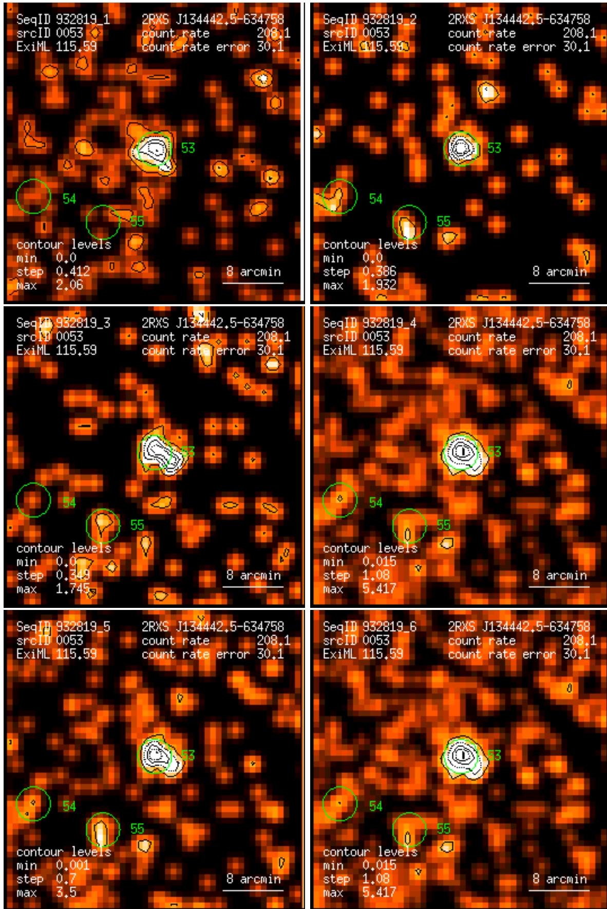
Figure 53: RASS 932819: detection 0053: band rate images, Gaussian filter: (1) PSPC channels 11 – 41, (2) 52 – 90, (3) 91 – 201, (4) 11 – 235, (5) 52 – 201, (6) 11 – 201. Broad band rates in counts/ks. Band rate contour levels in counts/ks/arcmin 2 .
