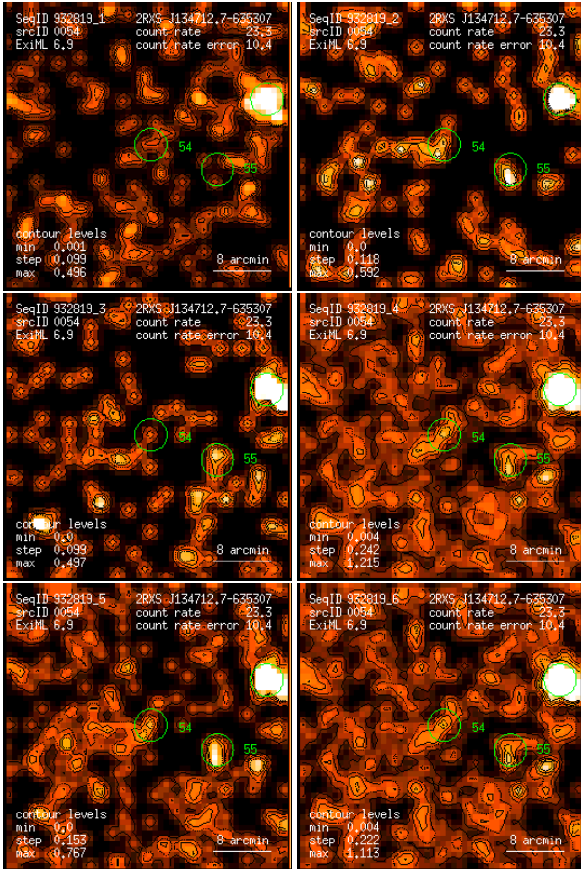
Figure 54: RASS 932819: detection 0054: band rate images, Gaussian filter: (1) PSPC channels 11 – 41, (2) 52 – 90, (3) 91 – 201, (4) 11 – 235, (5) 52 – 201, (6) 11 – 201. Broad band rates in counts/ks. Band rate contour levels in counts/ks/arcmin 2 .
