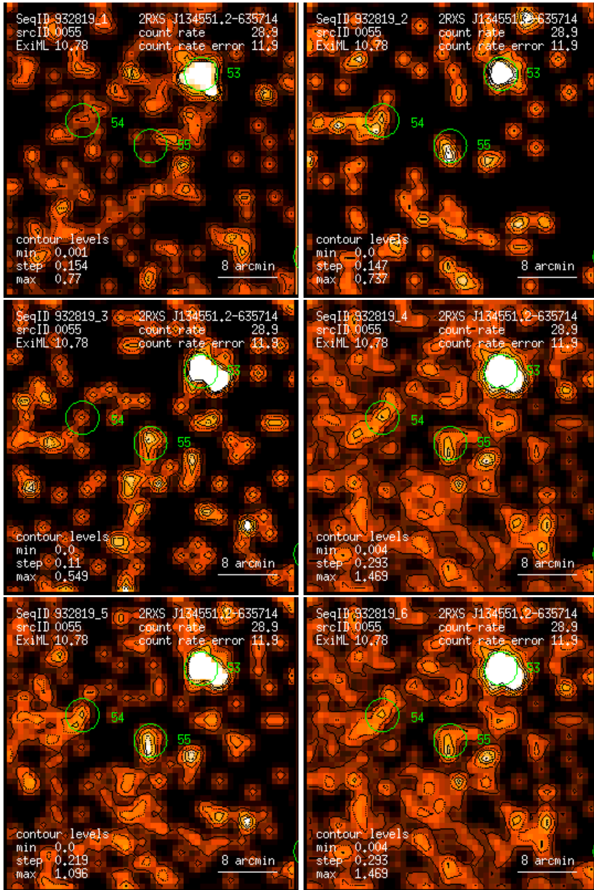
Figure 55: RASS 932819: detection 0055: band rate images, Gaussian filter: (1) PSPC channels 11 – 41, (2) 52 – 90, (3) 91 – 201, (4) 11 – 235, (5) 52 – 201, (6) 11 – 201. Broad band rates in counts/ks. Band rate contour levels in counts/ks/arcmin 2 .
