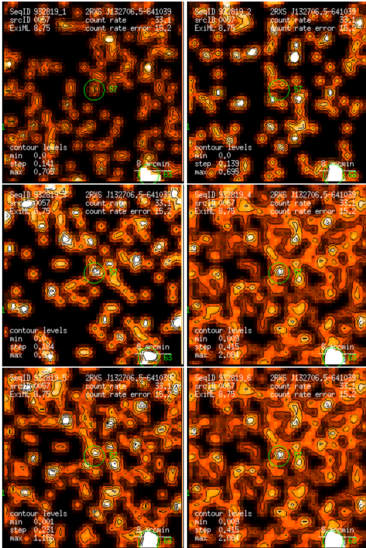
Figure 57: RASS 932819: detection 0057: band rate images, Gaussian filter: (1) PSPC channels 11 – 41, (2) 52 – 90, (3) 91 – 201, (4) 11 – 235, (5) 52 – 201, (6) 11 – 201. Broad band rates in counts/ks. Band rate contour levels in counts/ks/arcmin 2 .
