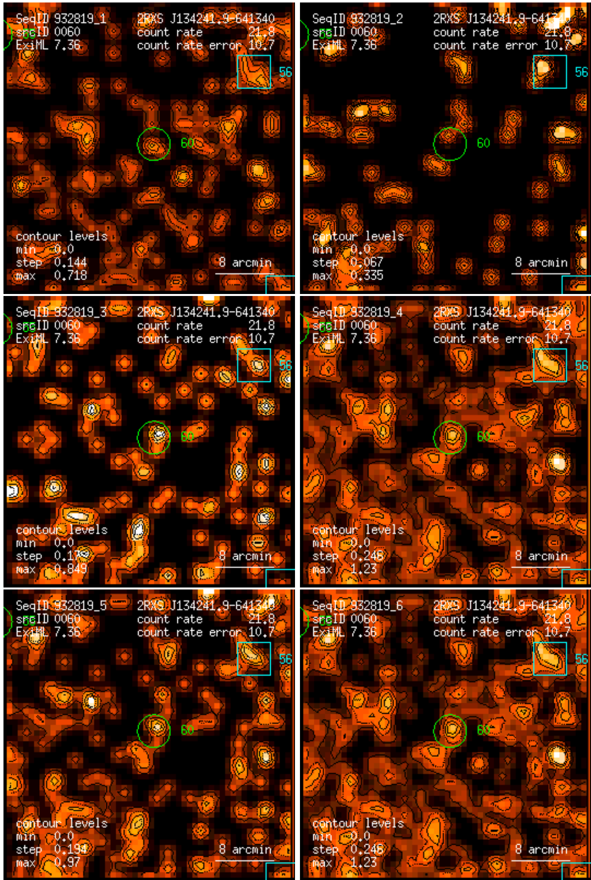
Figure 60: RASS 932819: detection 0060: band rate images, Gaussian filter: (1) PSPC channels 11 – 41, (2) 52 – 90, (3) 91 – 201, (4) 11 – 235, (5) 52 – 201, (6) 11 – 201. Broad band rates in counts/ks. Band rate contour levels in counts/ks/arcmin 2 .
